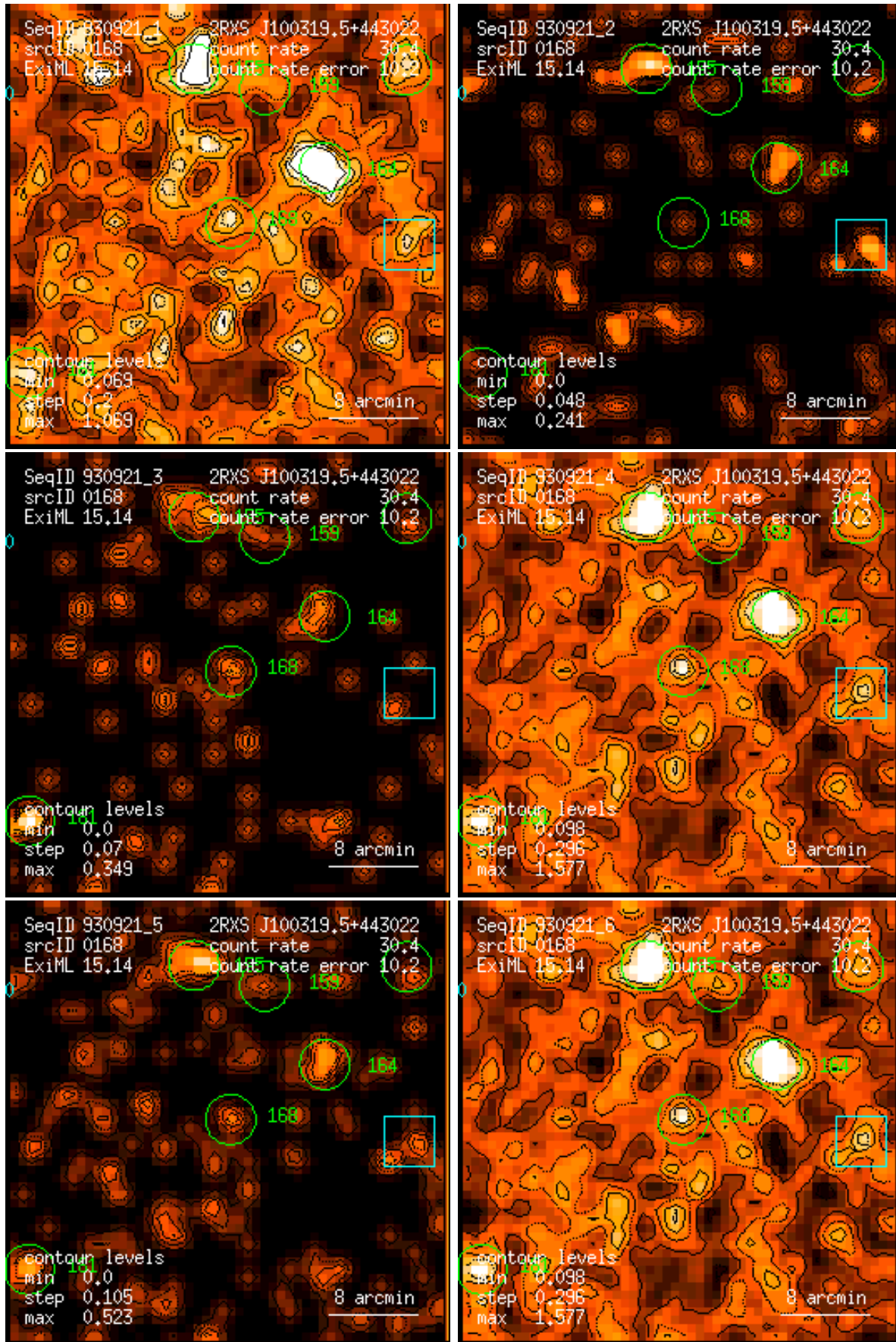
Figure 168: RASS 930921: detection 0168: band rate images, Gaussian filter: (1) PSPC channels 11 – 41, (2) 52 – 90, (3) 91 – 201, (4) 11 – 235, (5) 52 – 201, (6) 11 – 201. Broad band rates in counts/ks. Band rate contour levels in counts/ks/arcmin 2 .
