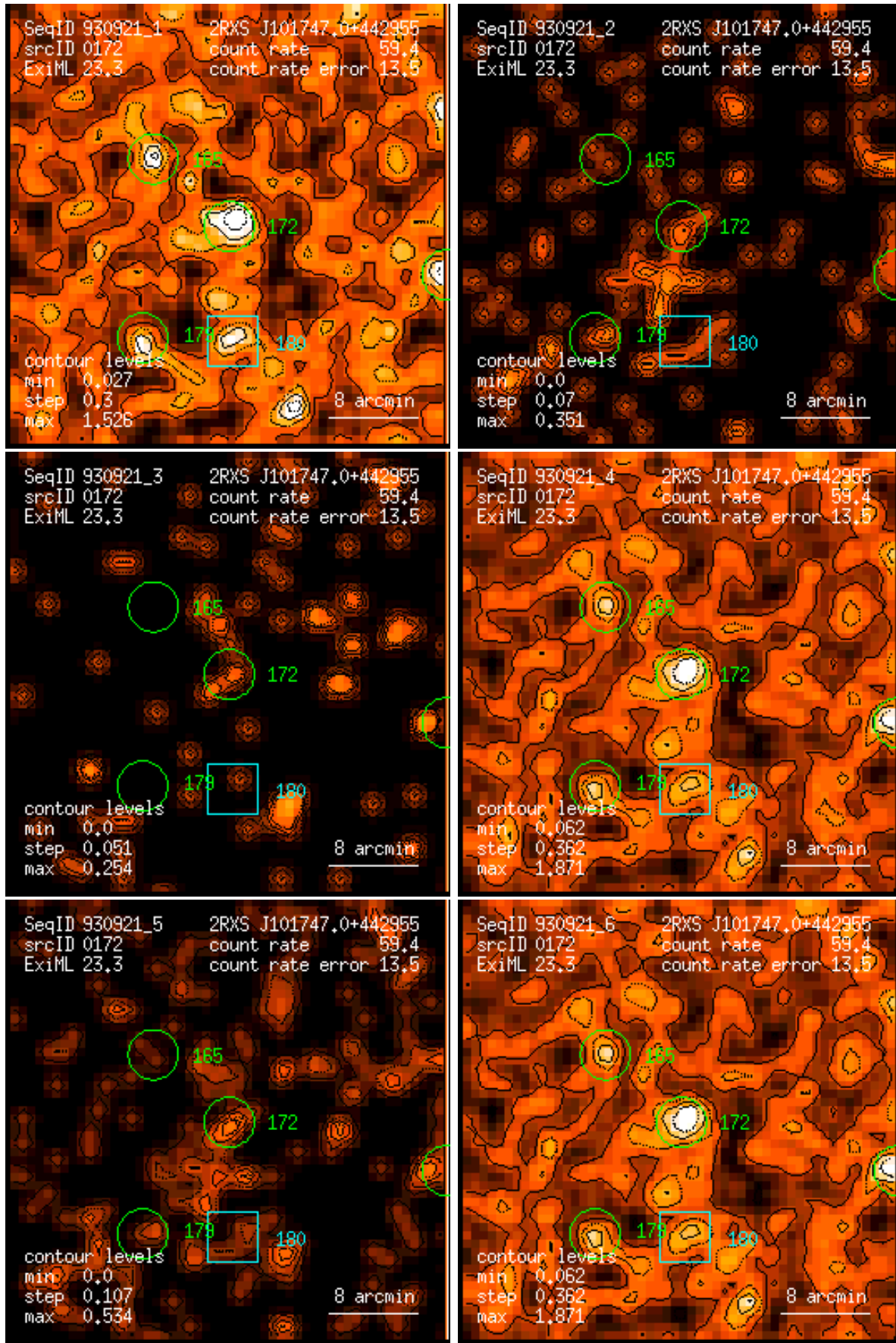
Figure 172: RASS 930921: detection 0172: band rate images, Gaussian filter: (1) PSPC channels 11 – 41, (2) 52 – 90, (3) 91 – 201, (4) 11 – 235, (5) 52 – 201, (6) 11 – 201. Broad band rates in counts/ks. Band rate contour levels in counts/ks/arcmin 2 .
