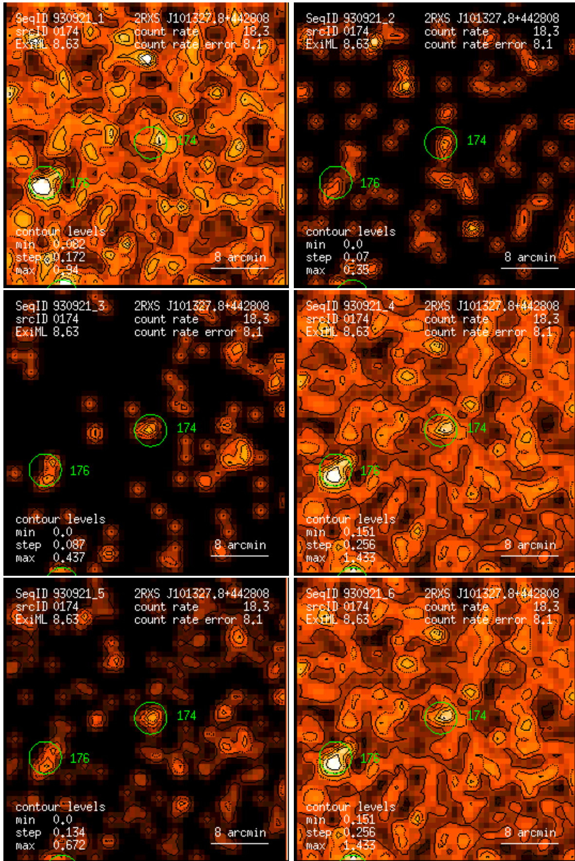
Figure 174: RASS 930921: detection 0174: band rate images, Gaussian filter: (1) PSPC channels 11 – 41, (2) 52 – 90, (3) 91 – 201, (4) 11 – 235, (5) 52 – 201, (6) 11 – 201. Broad band rates in counts/ks. Band rate contour levels in counts/ks/arcmin 2 .
