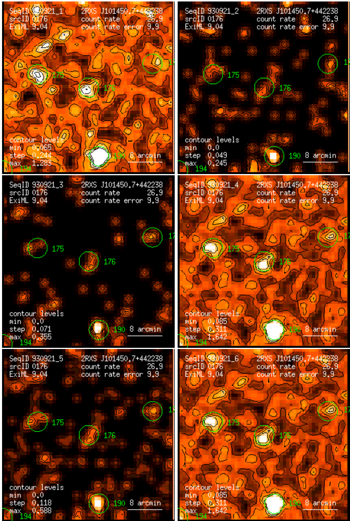
Figure 176: RASS 930921: detection 0176: band rate images, Gaussian filter: (1) PSPC channels 11 – 41, (2) 52 – 90, (3) 91 – 201, (4) 11 – 235, (5) 52 – 201, (6) 11 – 201. Broad band rates in counts/ks. Band rate contour levels in counts/ks/arcmin 2 .
