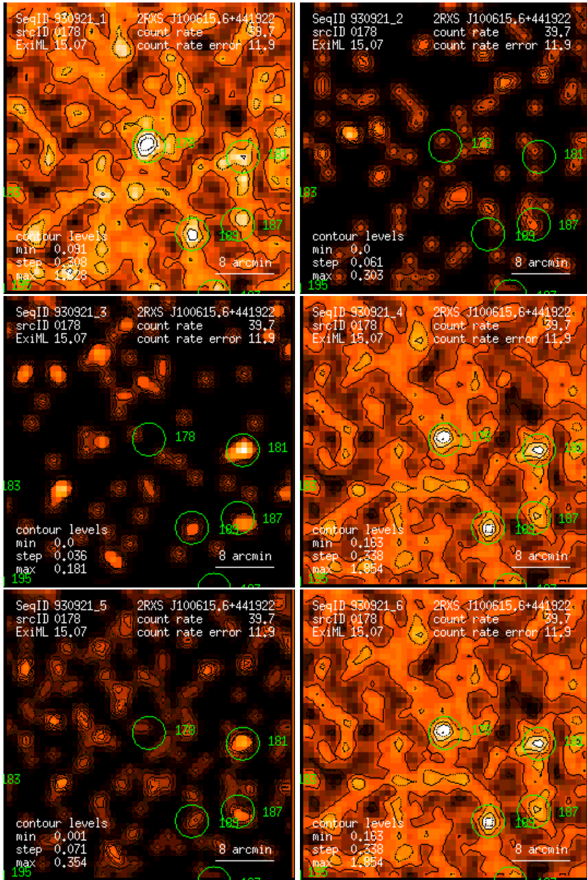
Figure 178: RASS 930921: detection 0178: band rate images, Gaussian filter: (1) PSPC channels 11 – 41, (2) 52 – 90, (3) 91 – 201, (4) 11 – 235, (5) 52 – 201, (6) 11 – 201. Broad band rates in counts/ks. Band rate contour levels in counts/ks/arcmin 2 .
