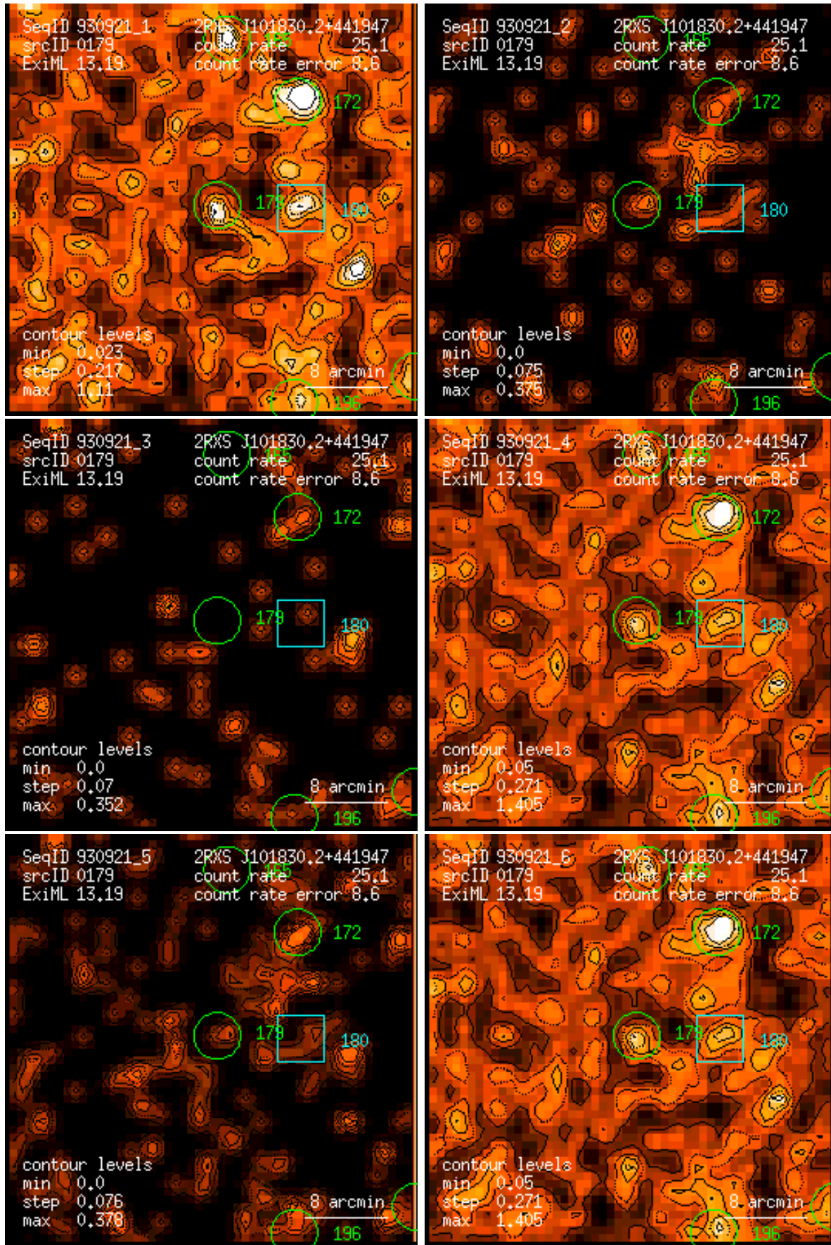
Figure 179: RASS 930921: detection 0179: band rate images, Gaussian filter: (1) PSPC channels 11 – 41, (2) 52 – 90, (3) 91 – 201, (4) 11 – 235, (5) 52 – 201, (6) 11 – 201. Broad band rates in counts/ks. Band rate contour levels in counts/ks/arcmin 2 .
