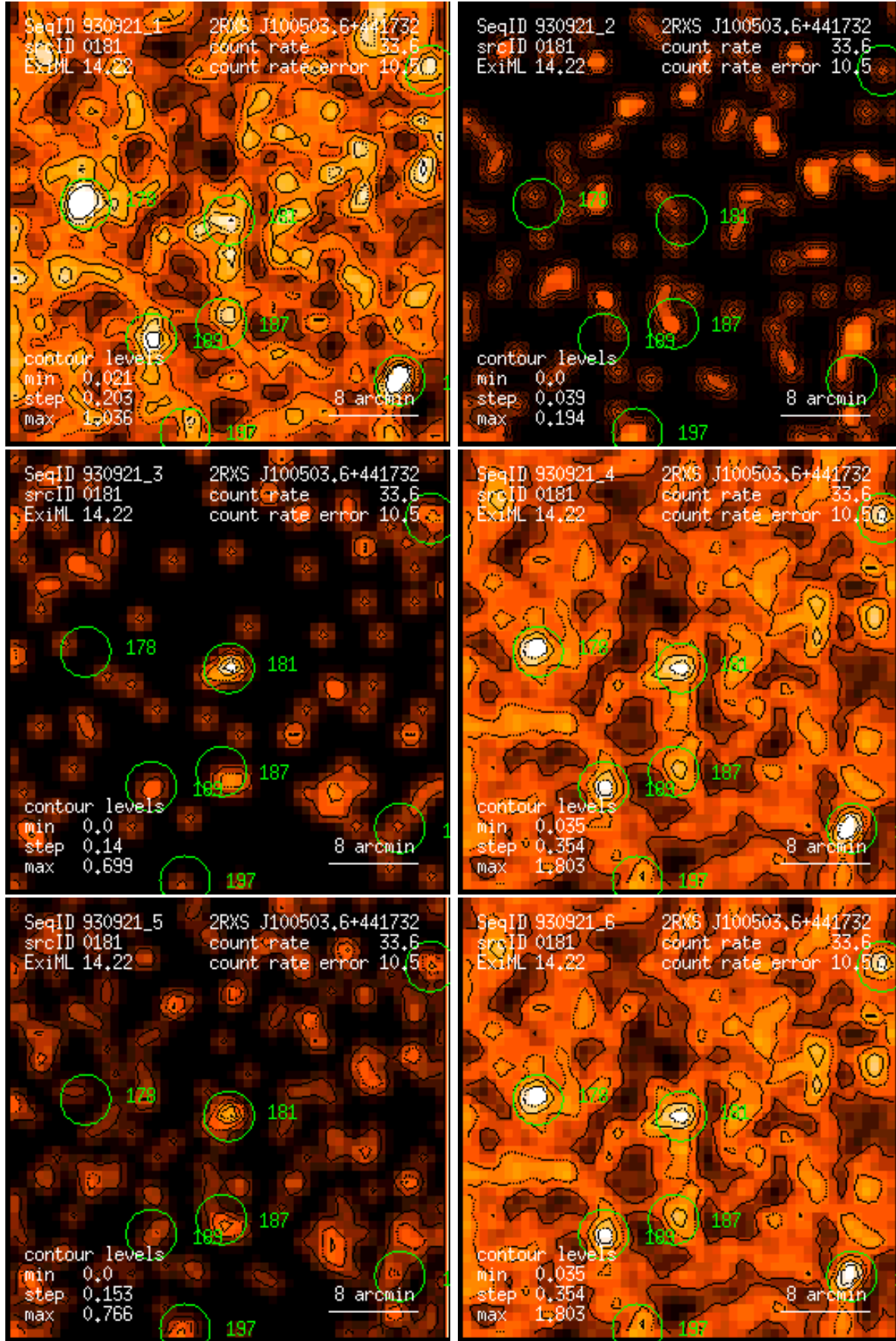
Figure 181: RASS 930921: detection 0181: band rate images, Gaussian filter: (1) PSPC channels 11 – 41, (2) 52 – 90, (3) 91 – 201, (4) 11 – 235, (5) 52 – 201, (6) 11 – 201. Broad band rates in counts/ks. Band rate contour levels in counts/ks/arcmin 2 .
