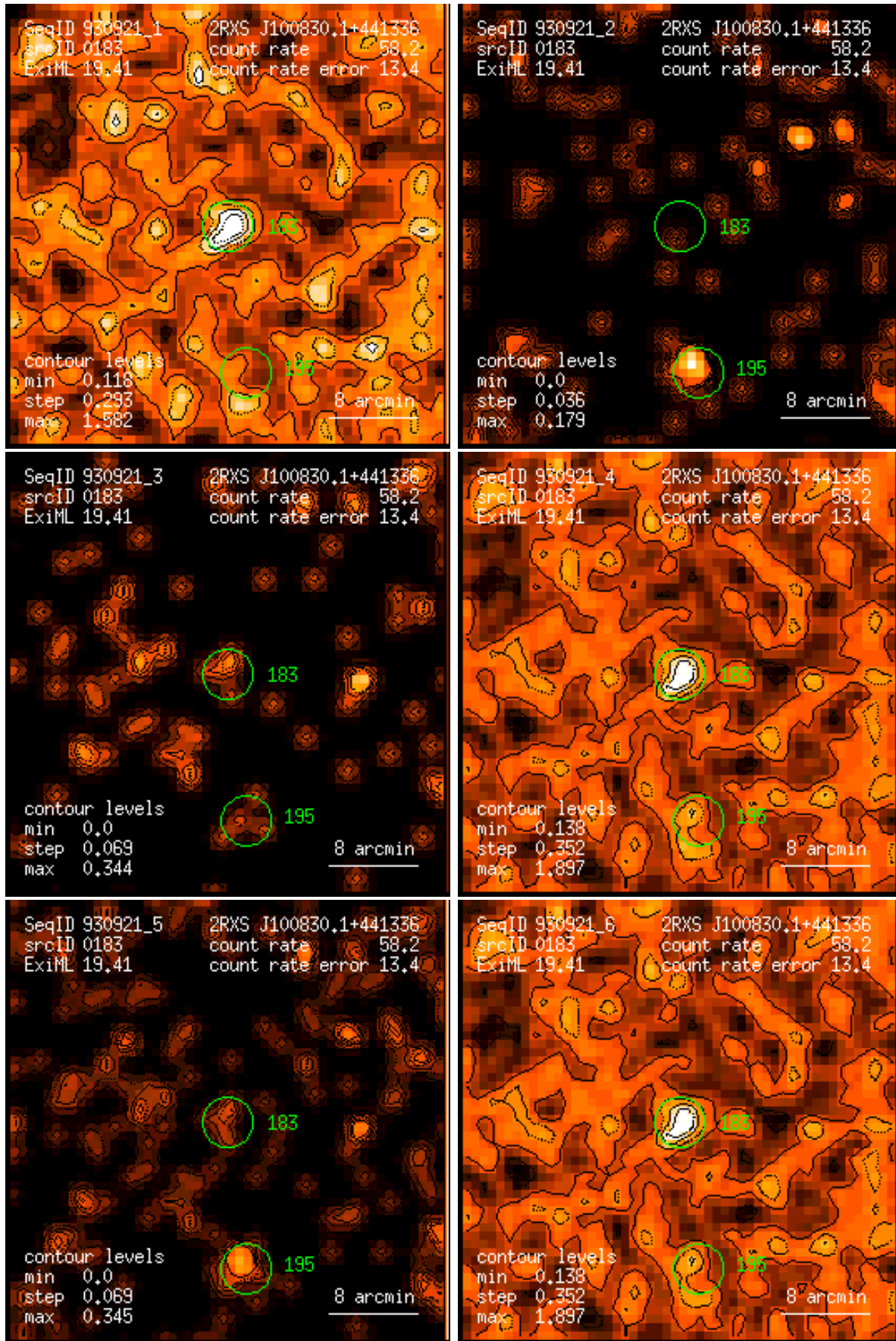
Figure 183: RASS 930921: detection 0183: band rate images, Gaussian filter: (1) PSPC channels 11 – 41, (2) 52 – 90, (3) 91 – 201, (4) 11 – 235, (5) 52 – 201, (6) 11 – 201. Broad band rates in counts/ks. Band rate contour levels in counts/ks/arcmin 2 .
