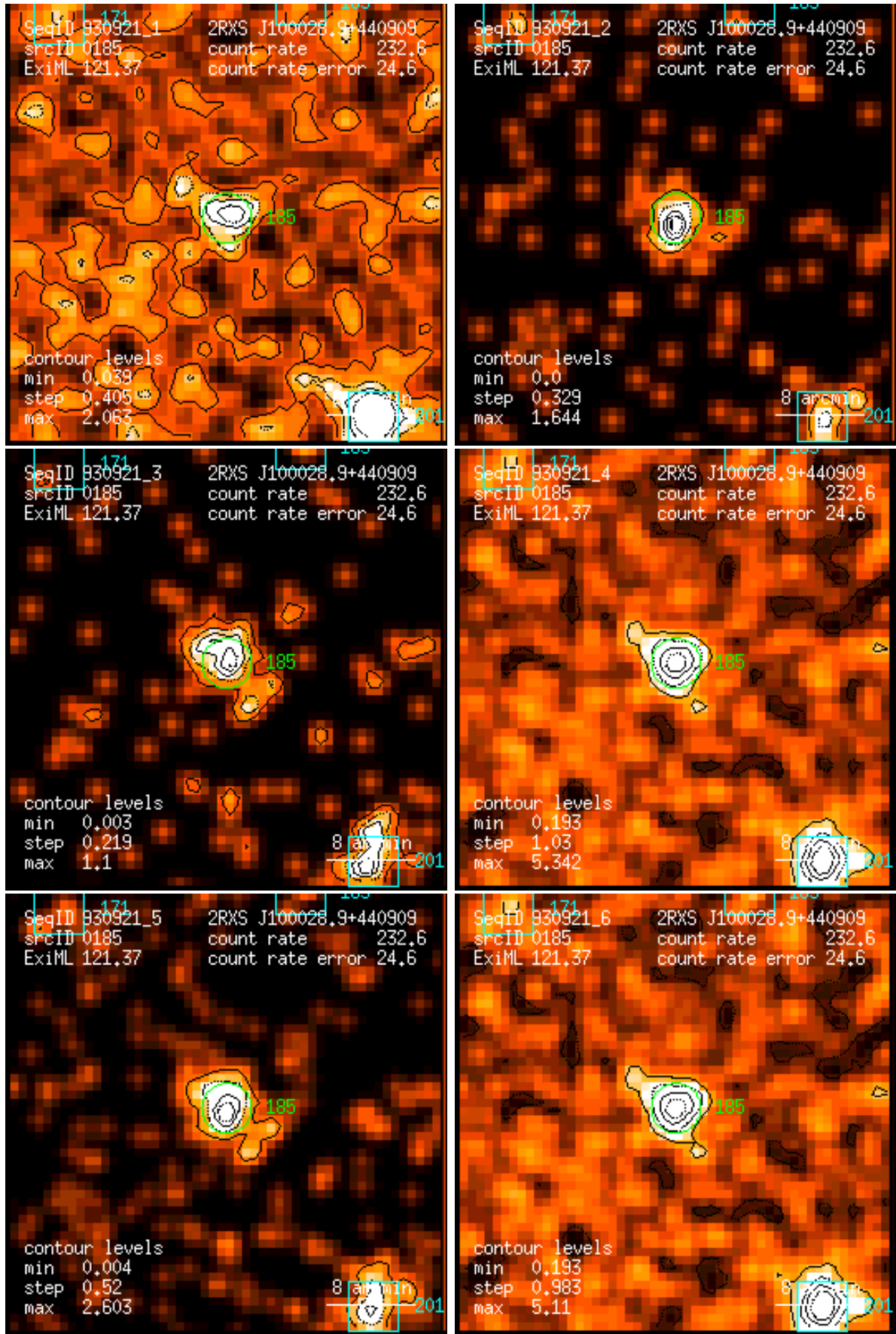
Figure 185: RASS 930921: detection 0185: band rate images, Gaussian filter: (1) PSPC channels 11 – 41, (2) 52 – 90, (3) 91 – 201, (4) 11 – 235, (5) 52 – 201, (6) 11 – 201. Broad band rates in counts/ks. Band rate contour levels in counts/ks/arcmin 2 .
