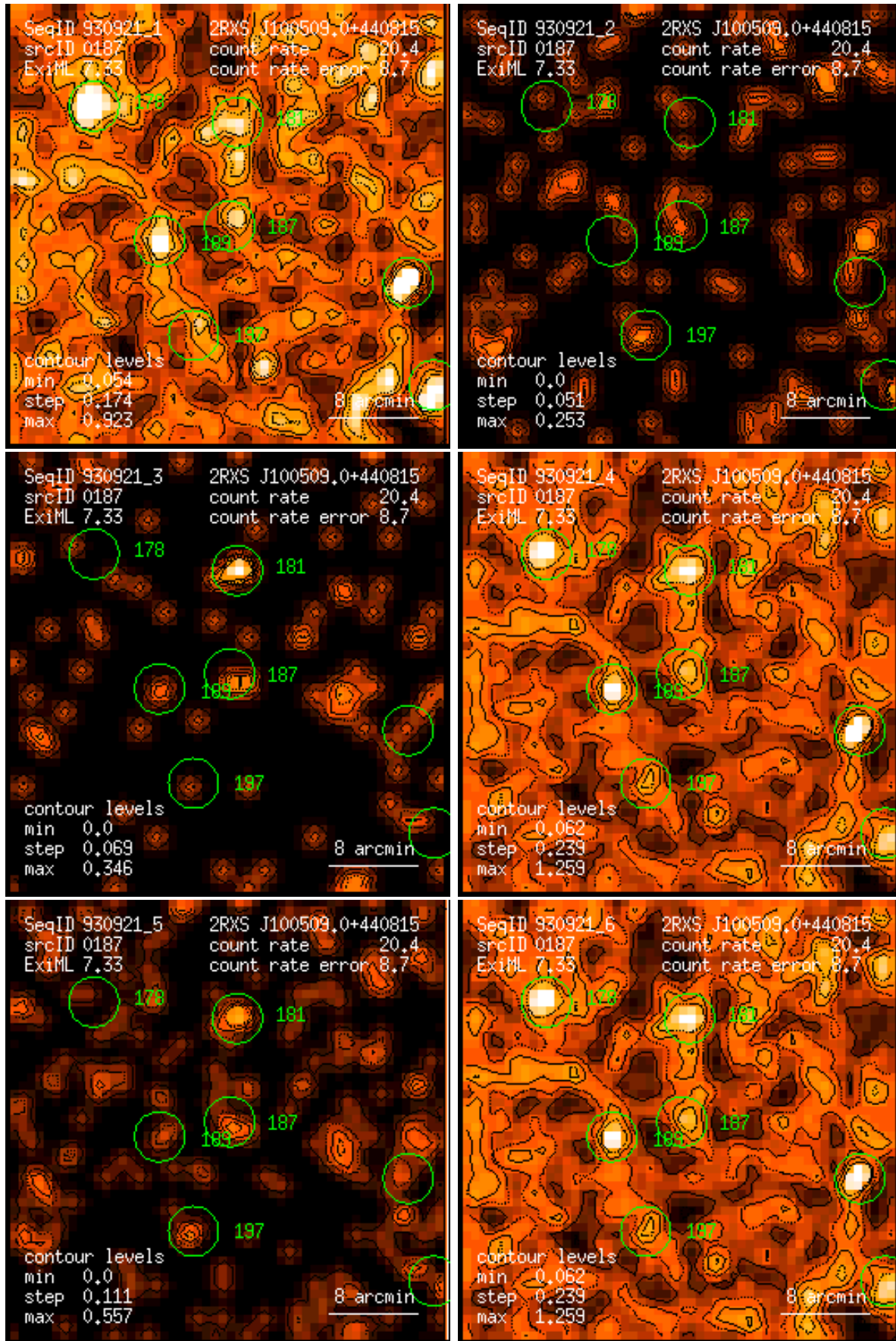
Figure 187: RASS 930921: detection 0187: band rate images, Gaussian filter: (1) PSPC channels 11 – 41, (2) 52 – 90, (3) 91 – 201, (4) 11 – 235, (5) 52 – 201, (6) 11 – 201. Broad band rates in counts/ks. Band rate contour levels in counts/ks/arcmin 2 .
