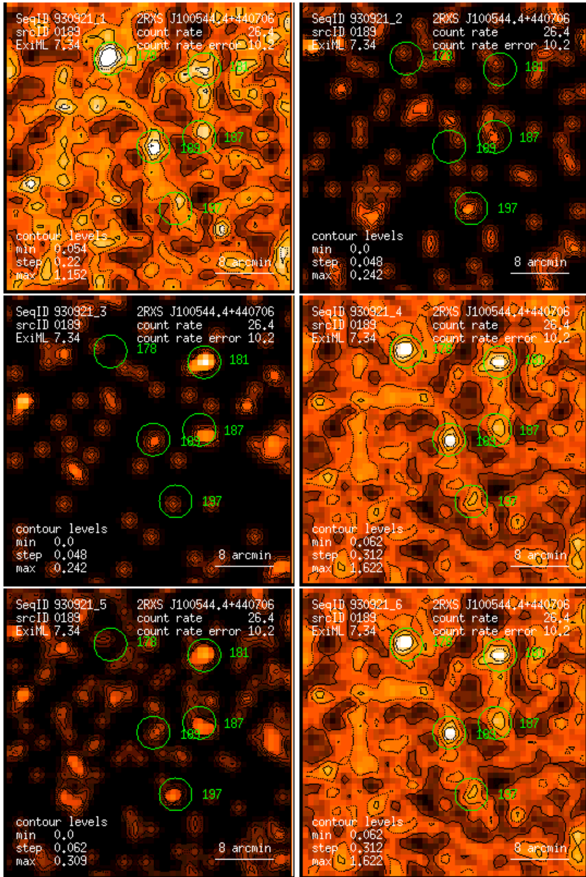
Figure 189: RASS 930921: detection 0189: band rate images, Gaussian filter: (1) PSPC channels 11 – 41, (2) 52 – 90, (3) 91 – 201, (4) 11 – 235, (5) 52 – 201, (6) 11 – 201. Broad band rates in counts/ks. Band rate contour levels in counts/ks/arcmin 2 .
