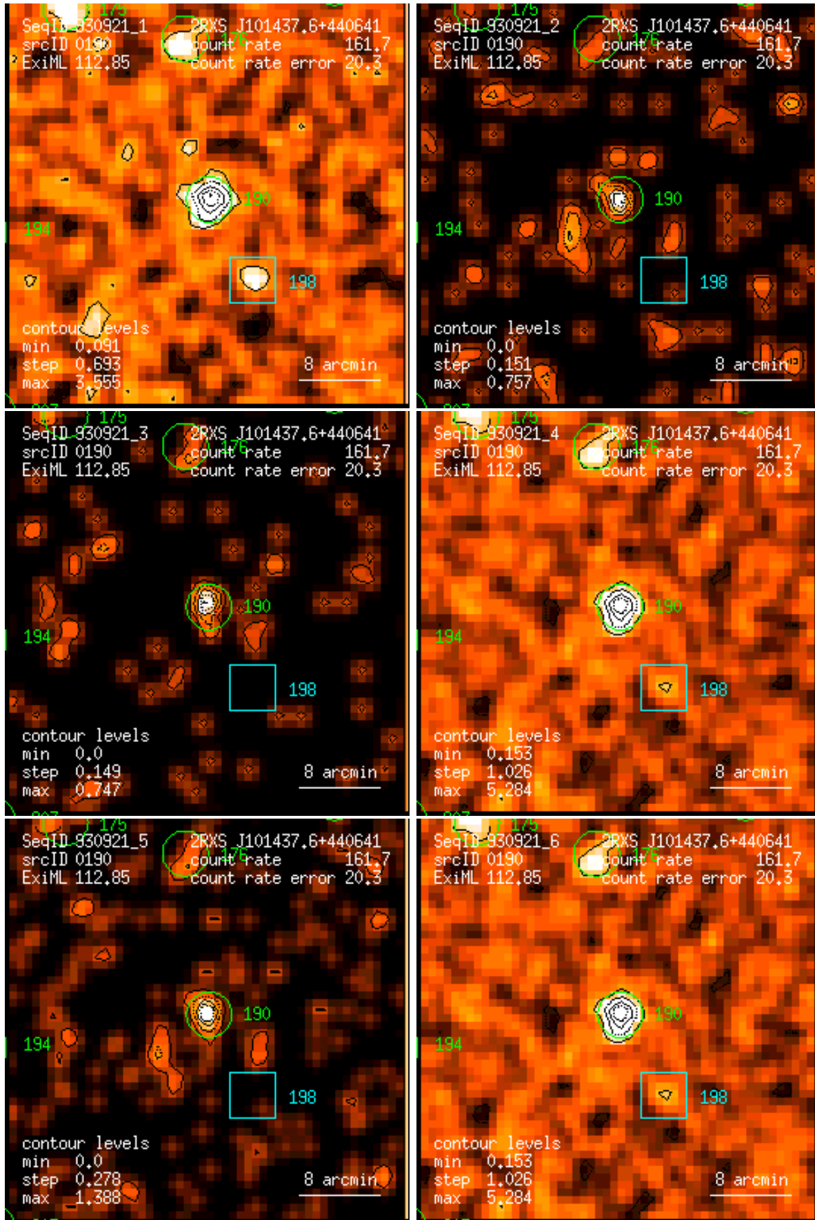
Figure 190: RASS 930921: detection 0190: band rate images, Gaussian filter: (1) PSPC channels 11 – 41, (2) 52 – 90, (3) 91 – 201, (4) 11 – 235, (5) 52 – 201, (6) 11 – 201. Broad band rates in counts/ks. Band rate contour levels in counts/ks/arcmin 2 .
