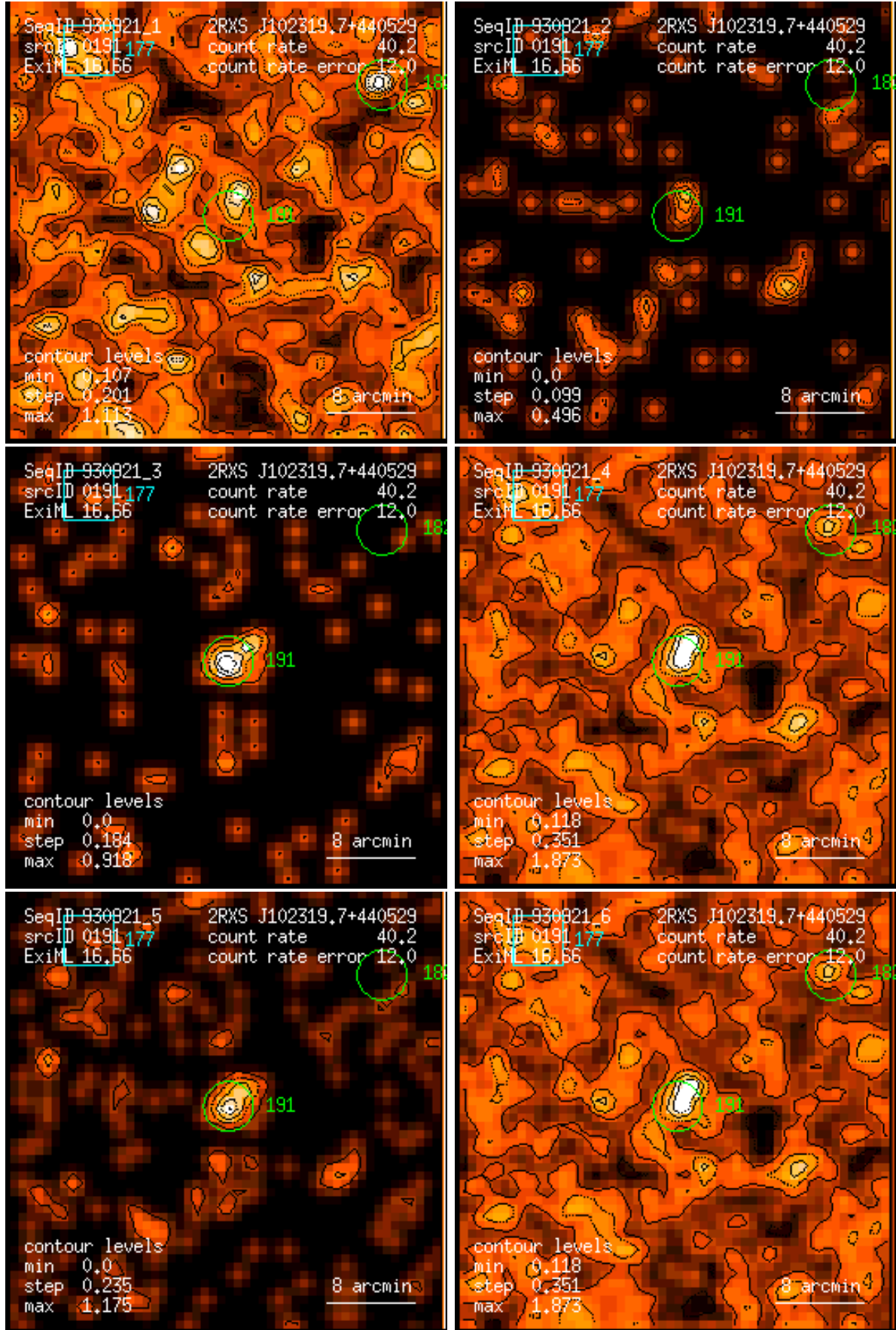
Figure 191: RASS 930921: detection 0191: band rate images, Gaussian filter: (1) PSPC channels 11 – 41, (2) 52 – 90, (3) 91 – 201, (4) 11 – 235, (5) 52 – 201, (6) 11 – 201. Broad band rates in counts/ks. Band rate contour levels in counts/ks/arcmin 2 .
