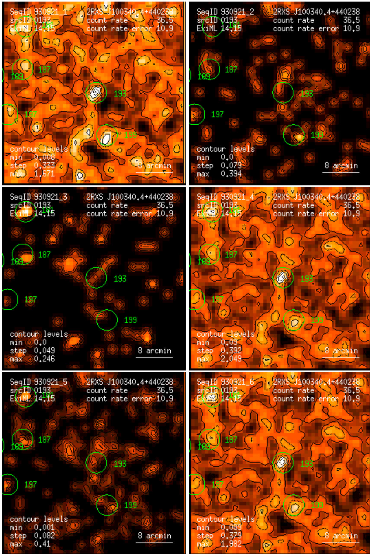
Figure 193: RASS 930921: detection 0193: band rate images, Gaussian filter: (1) PSPC channels 11 – 41, (2) 52 – 90, (3) 91 – 201, (4) 11 – 235, (5) 52 – 201, (6) 11 – 201. Broad band rates in counts/ks. Band rate contour levels in counts/ks/arcmin 2 .
