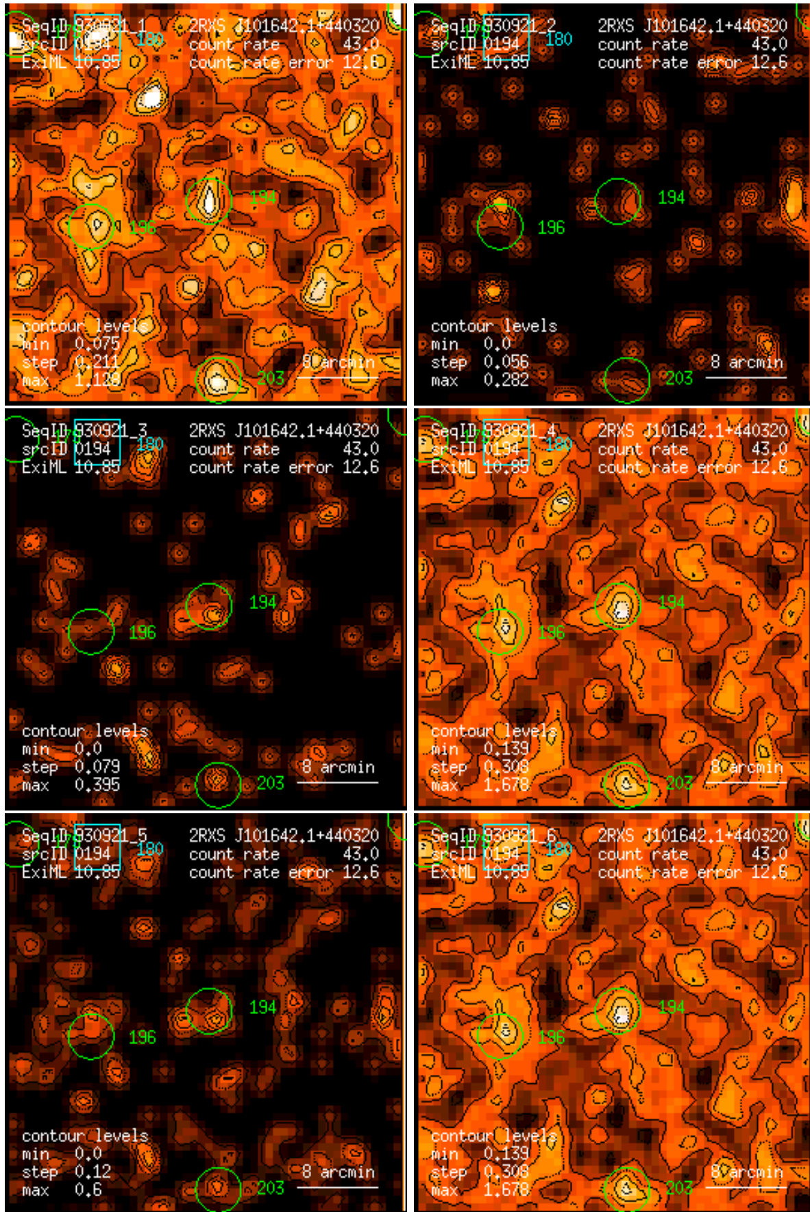
Figure 194: RASS 930921: detection 0194: band rate images, Gaussian filter: (1) PSPPC channels 11 – 41, (2) 52 – 90, (3) 91 – 201, (4) 11 – 235, (5) 52 – 201, (6) 11 – 201. Broad band rates in counts/ks. Band rate contour levels in counts/ks/arcmin 2 .
