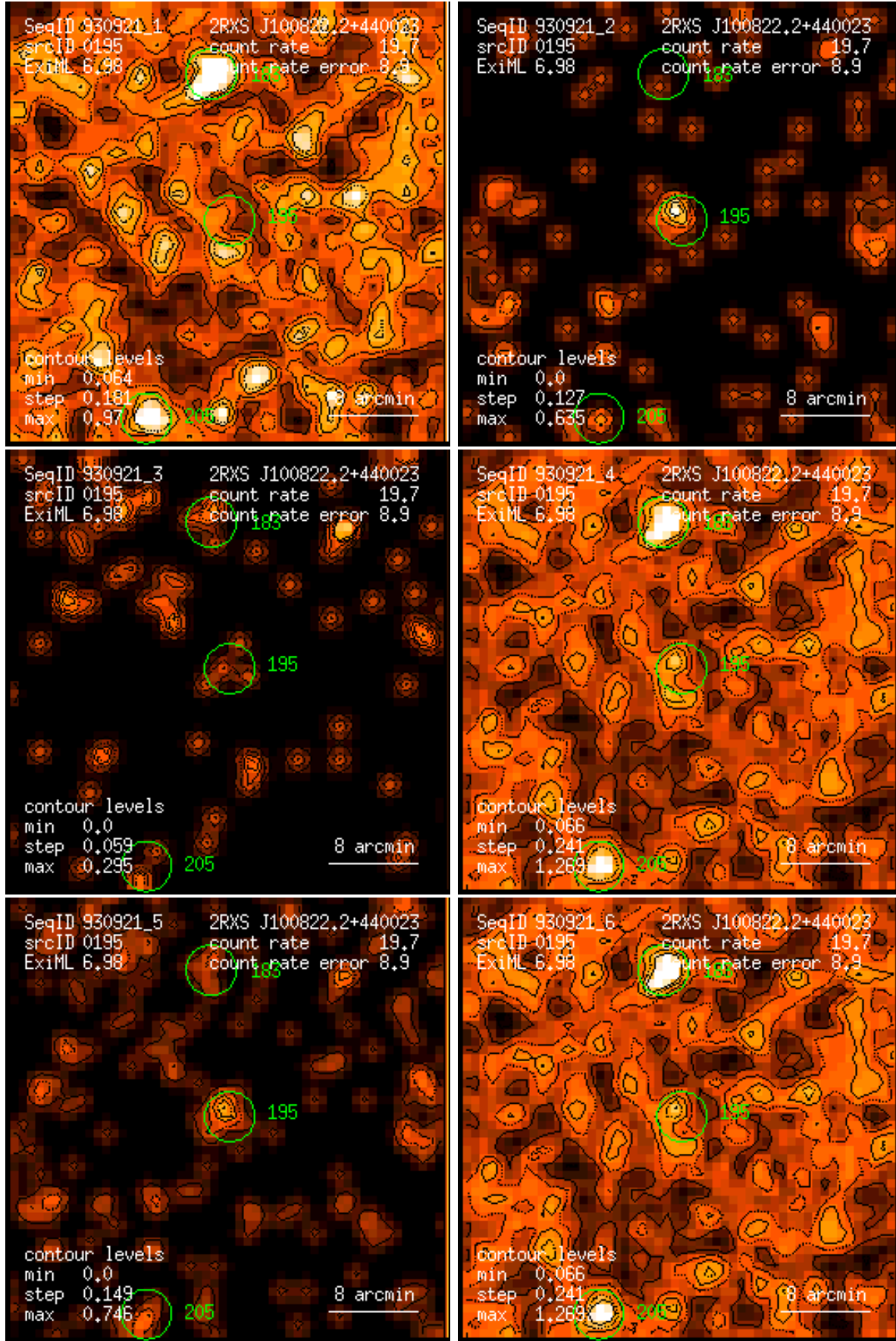
Figure 195: RASS 930921: detection 0195: band rate images, Gaussian filter: (1) PSPC channels 11 – 41, (2) 52 – 90, (3) 91 – 201, (4) 11 – 235, (5) 52 – 201, (6) 11 – 201. Broad band rates in counts/ks. Band rate contour levels in counts/ks/arcmin 2 .
