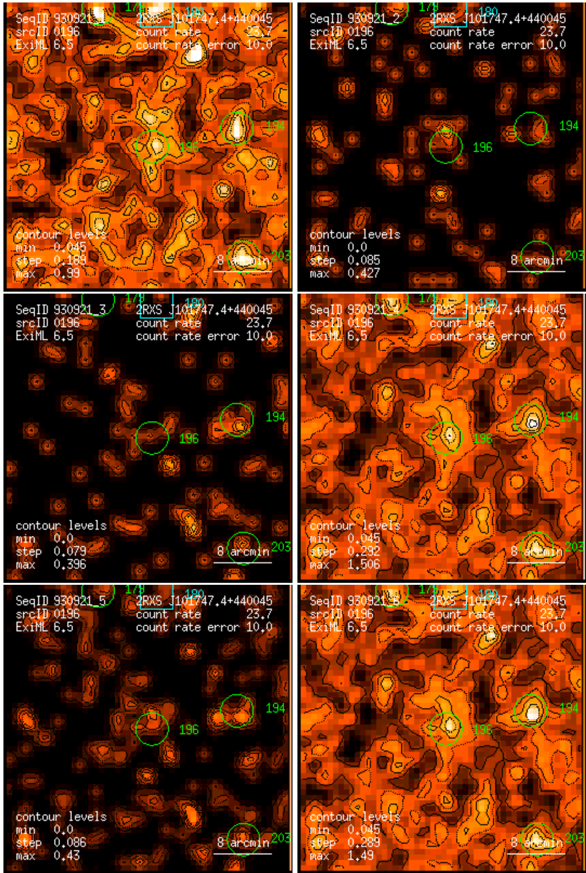
Figure 196: RASS 930921: detection 0196: band rate images, Gaussian filter: (1) PSPC channels 11 – 41, (2) 52 – 90, (3) 91 – 201, (4) 11 – 235, (5) 52 – 201, (6) 11 – 201. Broad band rates in counts/ks. Band rate contour levels in counts/ks/arcmin 2 .
