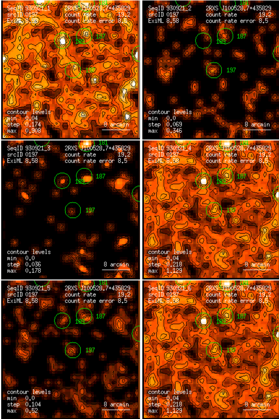
Figure 197: RASS 930921: detection 0197: band rate images, Gaussian filter: (1) PSPC channels 11 – 41, (2) 52 – 90, (3) 91 – 201, (4) 11 – 235, (5) 52 – 201, (6) 11 – 201. Broad band rates in counts/ks. Band rate contour levels in counts/ks/arcmin 2 .
