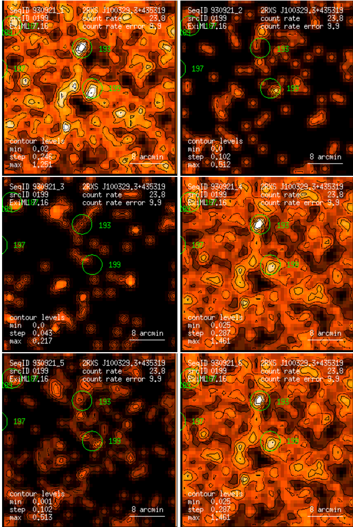
Figure 199: RASS 930921: detection 0199: band rate images, Gaussian filter: (1) PSPC channels 11 – 41, (2) 52 – 90, (3) 91 – 201, (4) 11 – 235, (5) 52 – 201, (6) 11 – 201. Broad band rates in counts/ks. Band rate contour levels in counts/ks/arcmin 2 .
