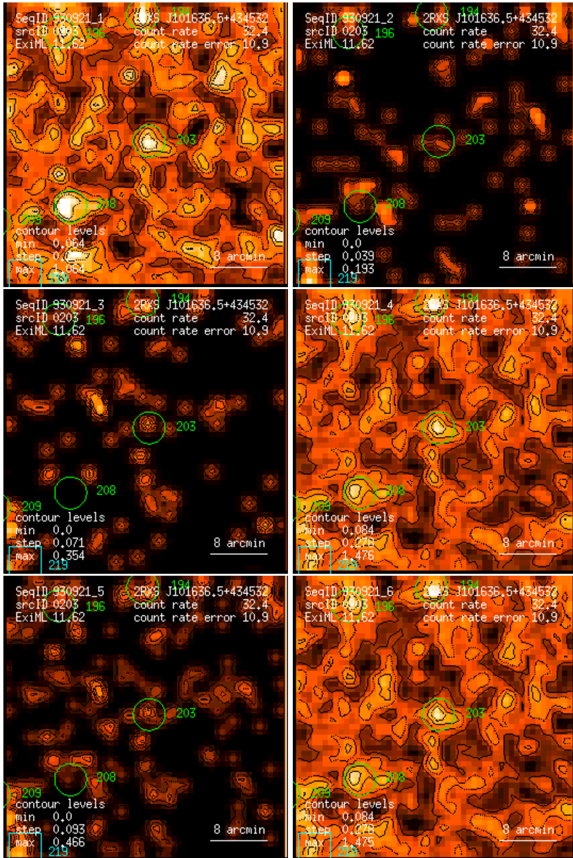
Figure 203: RASS 930921: detection 0203: band rate images, Gaussian filter: (1) PSPC channels 11 – 41, (2) 52 – 90, (3) 91 – 201, (4) 11 – 235, (5) 52 – 201, (6) 11 – 201. Broad band rates in counts/ks. Band rate contour levels in counts/ks/arcmin 2 .
