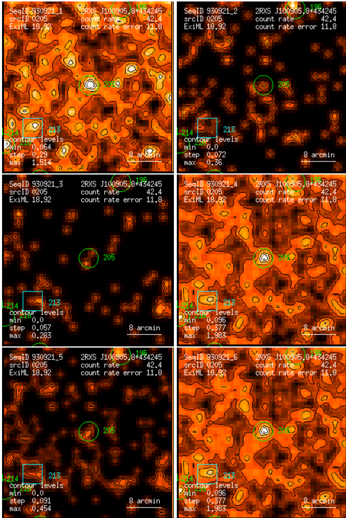
Figure 205: RASS 930921: detection 0205: band rate images, Gaussian filter: (1) PSPC channels 11 – 41, (2) 52 – 90, (3) 91 – 201, (4) 11 – 235, (5) 52 – 201, (6) 11 – 201. Broad band rates in counts/ks. Band rate contour levels in counts/ks/arcmin 2 .
