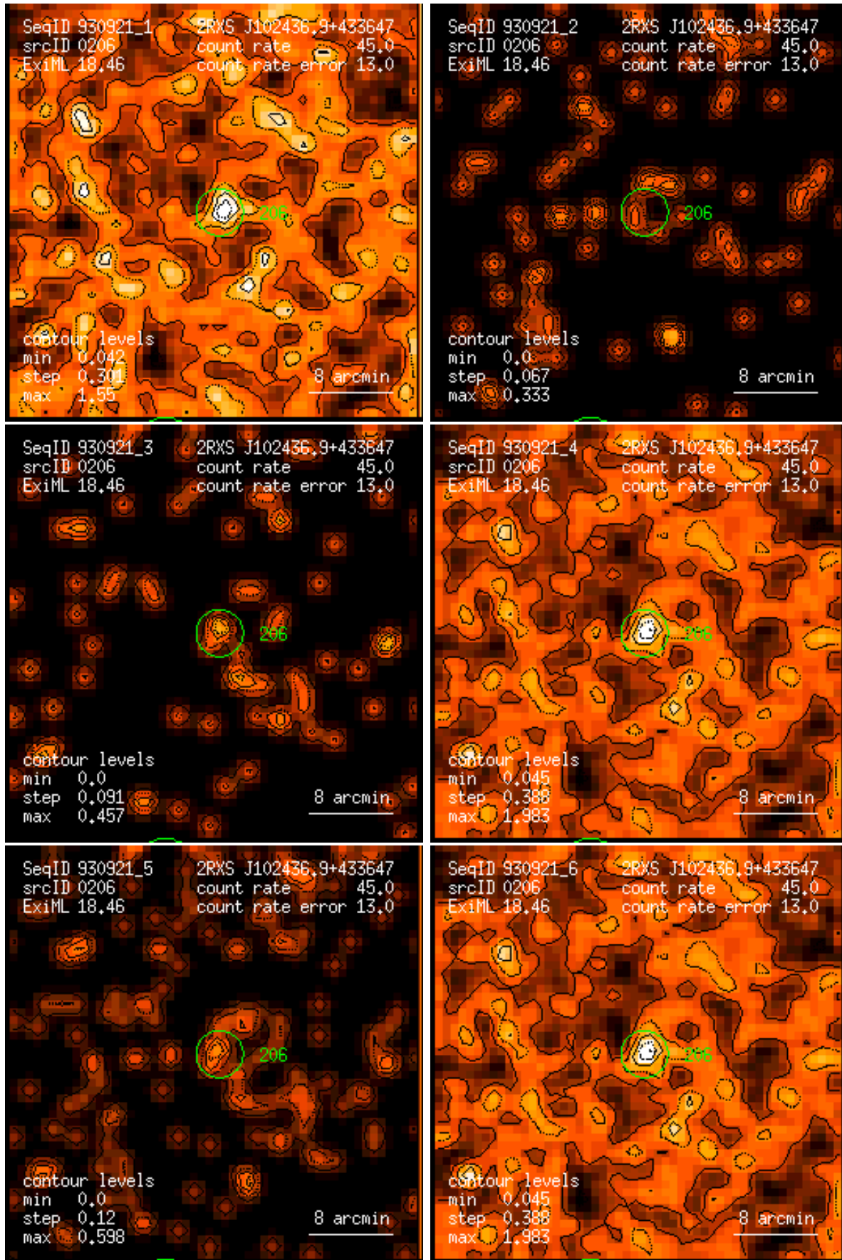
Figure 206: RASS 930921: detection 0206: band rate images, Gaussian filter: (1) PSPC channels 11 – 41, (2) 52 – 90, (3) 91 – 201, (4) 11 – 235, (5) 52 – 201, (6) 11 – 201. Broad band rates in counts/ks. Band rate contour levels in counts/ks/arcmin 2 .
