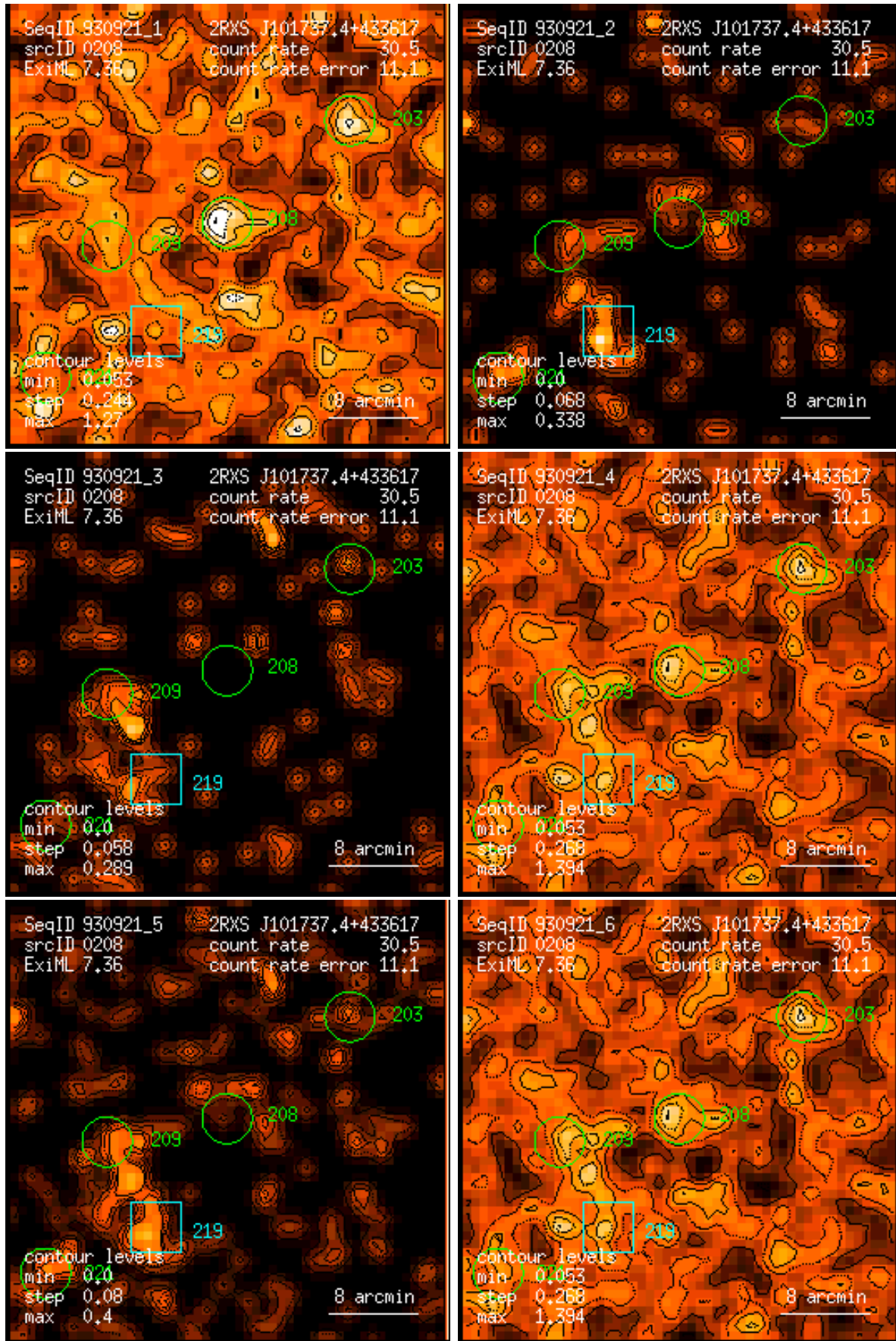
Figure 208: RASS 930921: detection 0208: band rate images, Gaussian filter: (1) PSPC channels 11 – 41, (2) 52 – 90, (3) 91 – 201, (4) 11 – 235, (5) 52 – 201, (6) 11 – 201. Broad band rates in counts/ks. Band rate contour levels in counts/ks/arcmin 2 .
