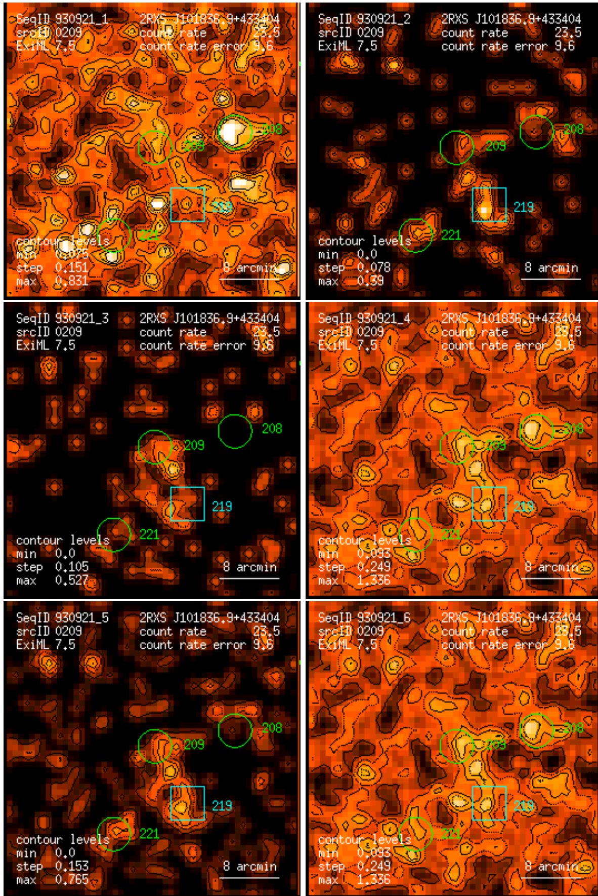
Figure 209: RASS 930921: detection 0209: band rate images, Gaussian filter: (1) PSPC channels 11 – 41, (2) 52 – 90, (3) 91 – 201, (4) 11 – 235, (5) 52 – 201, (6) 11 – 201. Broad band rates in counts/ks. Band rate contour levels in counts/ks/arcmin 2 .
