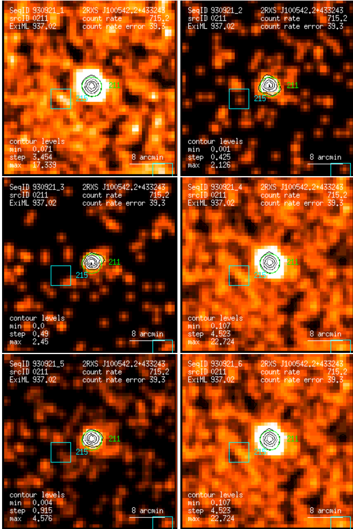
Figure 211: RASS 930921: detection 0211: band rate images, Gaussian filter: (1) PSPC channels 11 – 41, (2) 52 – 90, (3) 91 – 201, (4) 11 – 235, (5) 52 – 201, (6) 11 – 201. Broad band rates in counts/ks. Band rate contour levels in counts/ks/arcmin 2 .
