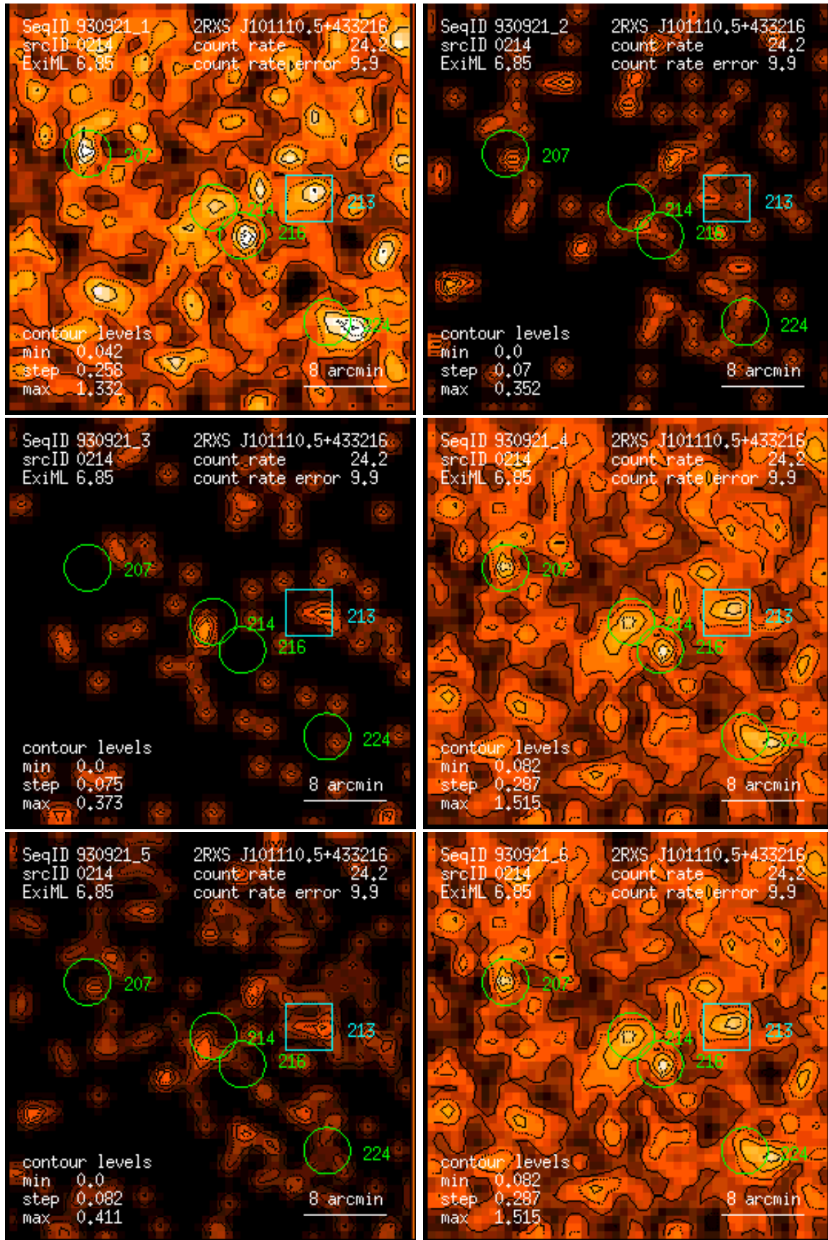
Figure 214: RASS 930921: detection 0214: band rate images, Gaussian filter: (1) PSPC channels 11 – 41, (2) 52 – 90, (3) 91 – 201, (4) 11 – 235, (5) 52 – 201, (6) 11 – 201. Broad band rates in counts/ks. Band rate contour levels in counts/ks/arcmin 2 .
