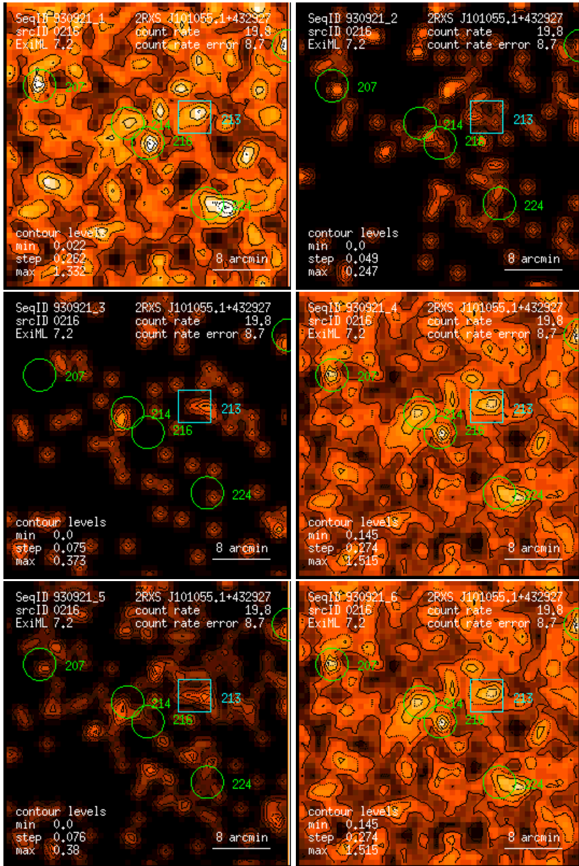
Figure 216: RASS 930921: detection 0216: band rate images, Gaussian filter: (1) PSPC channels 11 – 41, (2) 52 – 90, (3) 91 – 201, (4) 11 – 235, (5) 52 – 201, (6) 11 – 201. Broad band rates in counts/ks. Band rate contour levels in counts/ks/arcmin 2 .
