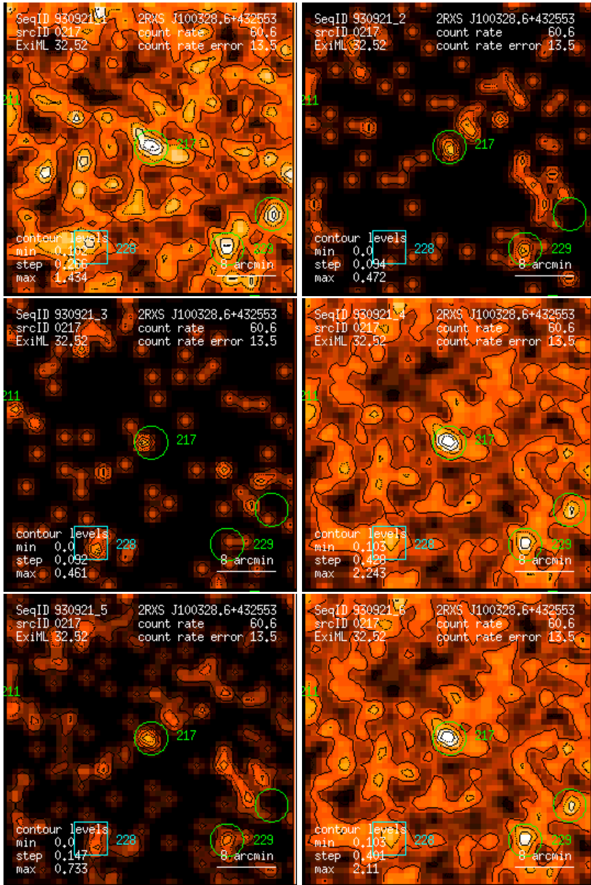
Figure 217: RASS 930921: detection 0217: band rate images, Gaussian filter: (1) PSPC channels 11 – 41, (2) 52 – 90, (3) 91 – 201, (4) 11 – 235, (5) 52 – 201, (6) 11 – 201. Broad band rates in counts/ks. Band rate contour levels in counts/ks/arcmin 2 .
