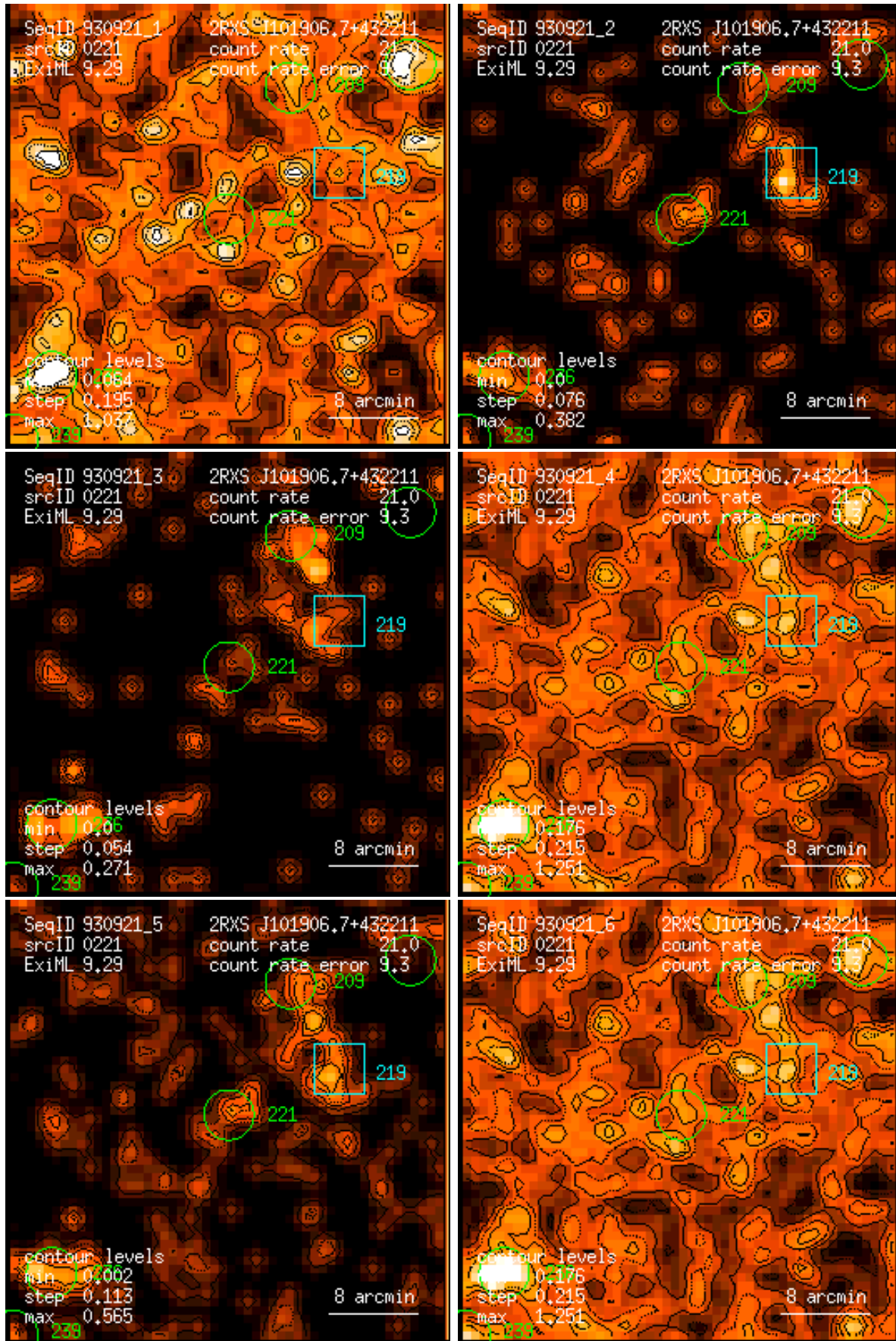
Figure 221: RASS 930921: detection 0221: band rate images, Gaussian filter: (1) PSPC channels 11 – 41, (2) 52 – 90, (3) 91 – 201, (4) 11 – 235, (5) 52 – 201, (6) 11 – 201. Broad band rates in counts/ks. Band rate contour levels in counts/ks/arcmin 2 .
