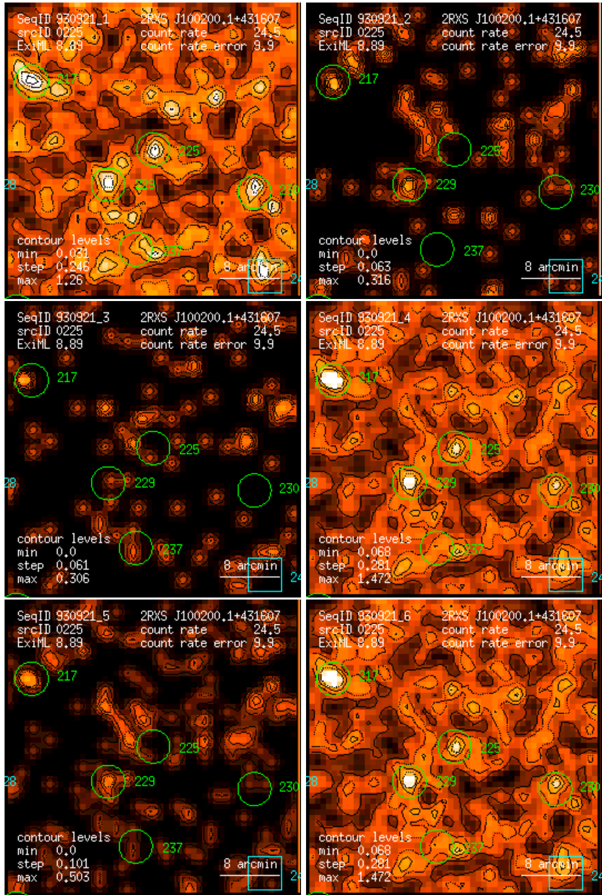
Figure 225: RASS 930921: detection 0225: band rate images, Gaussian filter: (1) PSPC channels 11 – 41, (2) 52 – 90, (3) 91 – 201, (4) 11 – 235, (5) 52 – 201, (6) 11 – 201. Broad band rates in counts/ks. Band rate contour levels in counts/ks/arcmin 2 .
