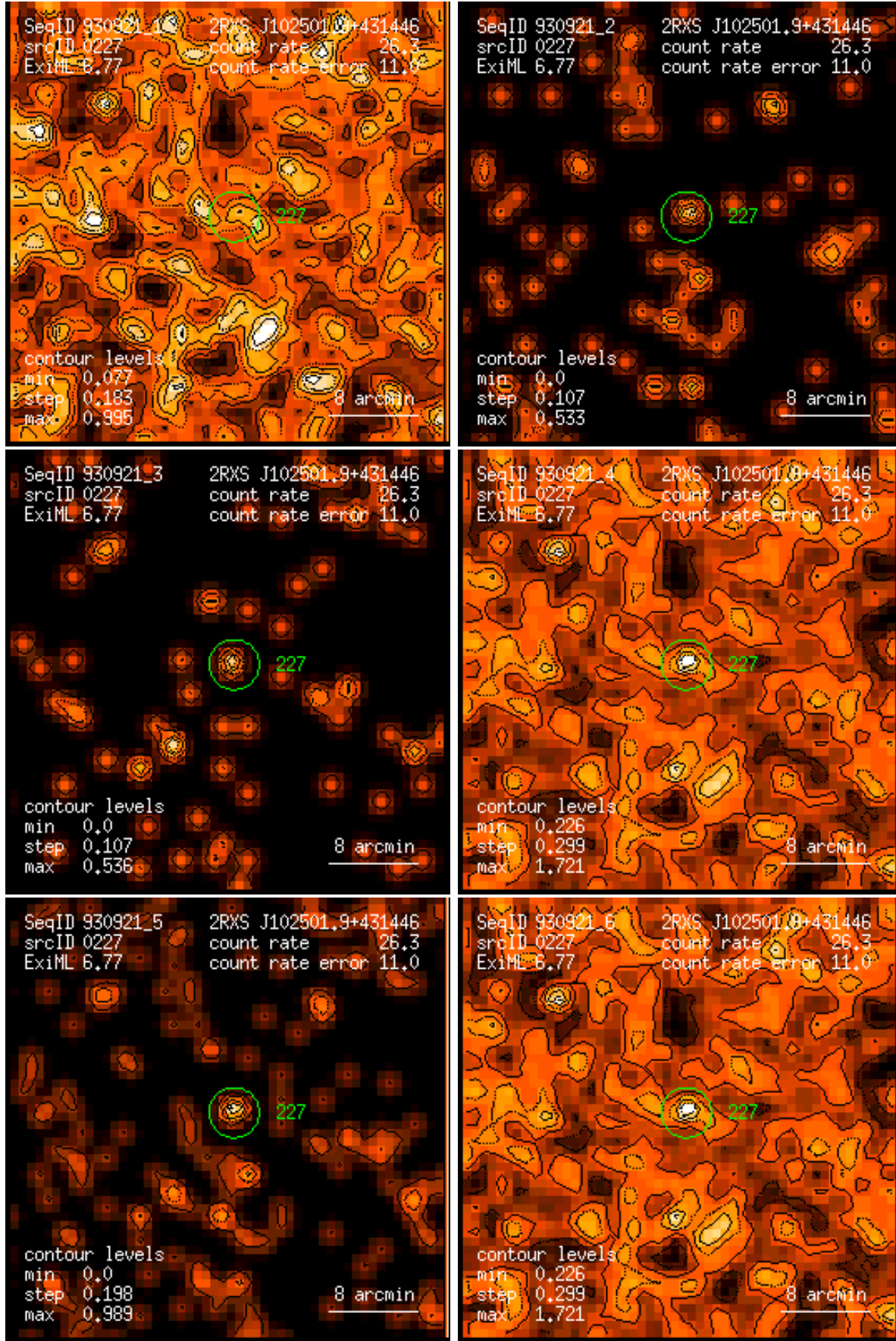
Figure 227: RASS 930921: detection 0227: band rate images, Gaussian filter: (1) PSPC channels 11 – 41, (2) 52 – 90, (3) 91 – 201, (4) 11 – 235, (5) 52 – 201, (6) 11 – 201. Broad band rates in counts/ks. Band rate contour levels in counts/ks/arcmin 2 .
