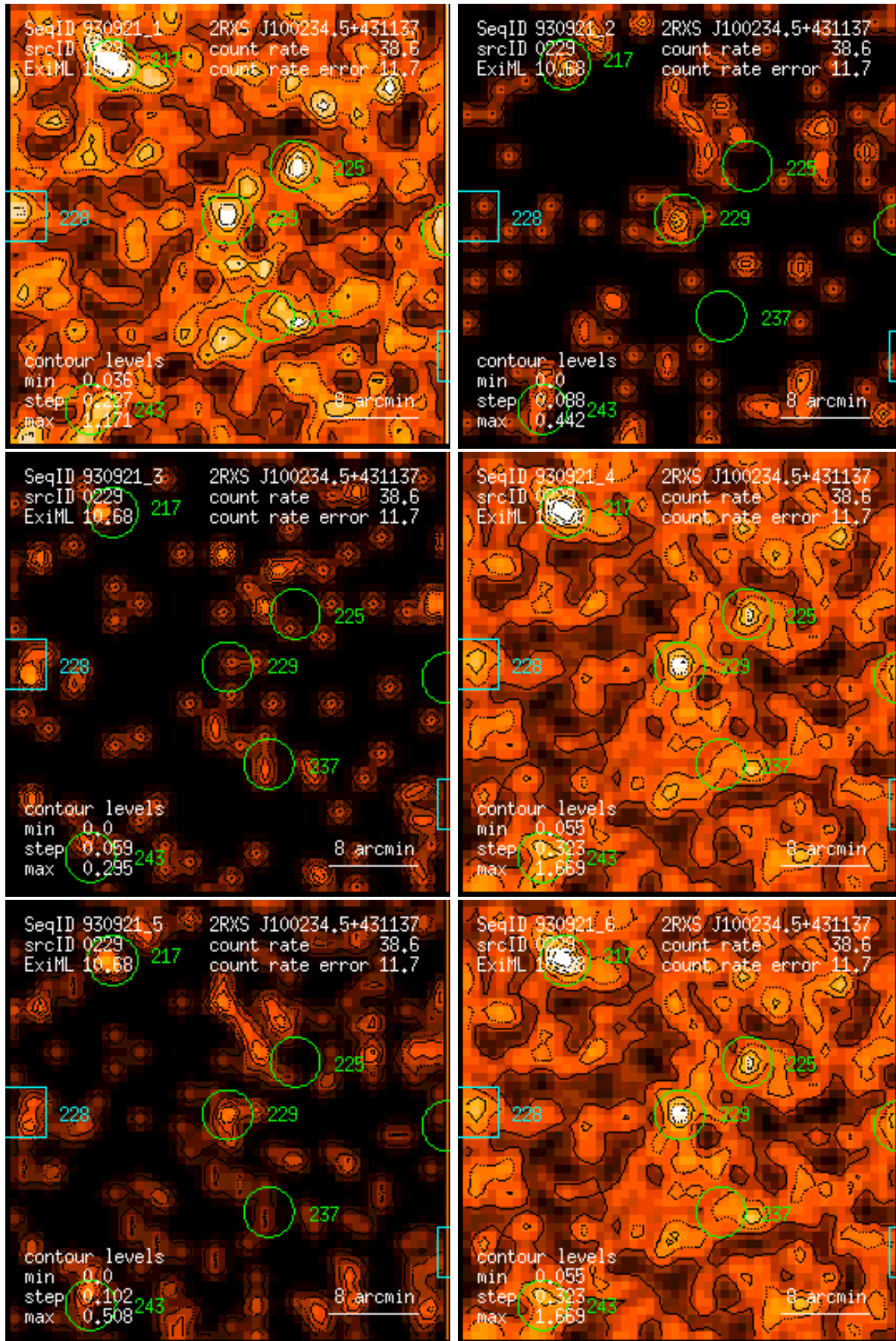
Figure 229: RASS 930921: detection 0229: band rate images, Gaussian filter: (1) PSPC channels 11 – 41, (2) 52 – 90, (3) 91 – 201, (4) 11 – 235, (5) 52 – 201, (6) 11 – 201. Broad band rates in counts/ks. Band rate contour levels in counts/ks/arcmin 2 .
