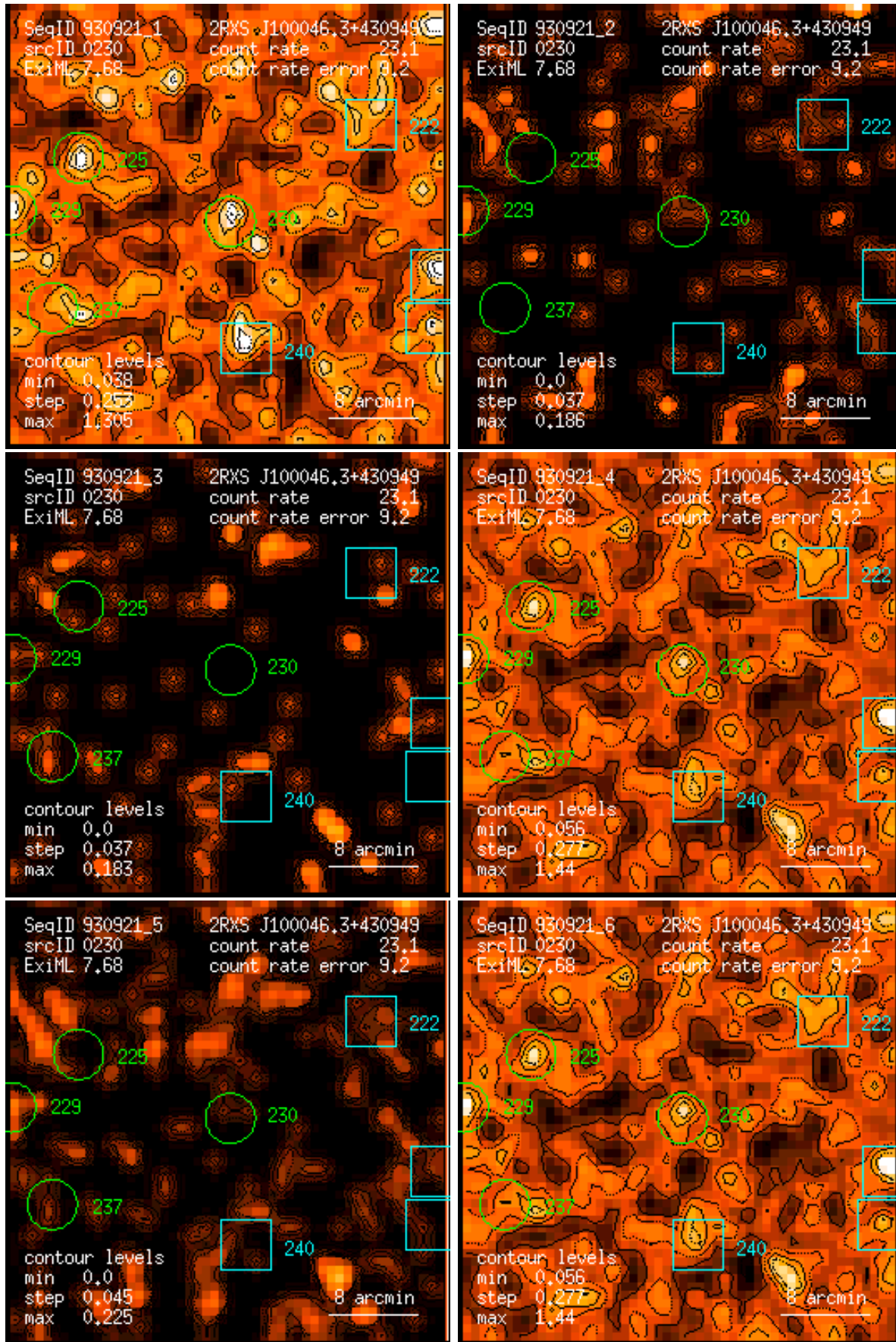
Figure 230: RASS 930921: detection 0230: band rate images, Gaussian filter: (1) PSPC channels 11 – 41, (2) 52 – 90, (3) 91 – 201, (4) 11 – 235, (5) 52 – 201, (6) 11 – 201. Broad band rates in counts/ks. Band rate contour levels in counts/ks/arcmin 2 .
