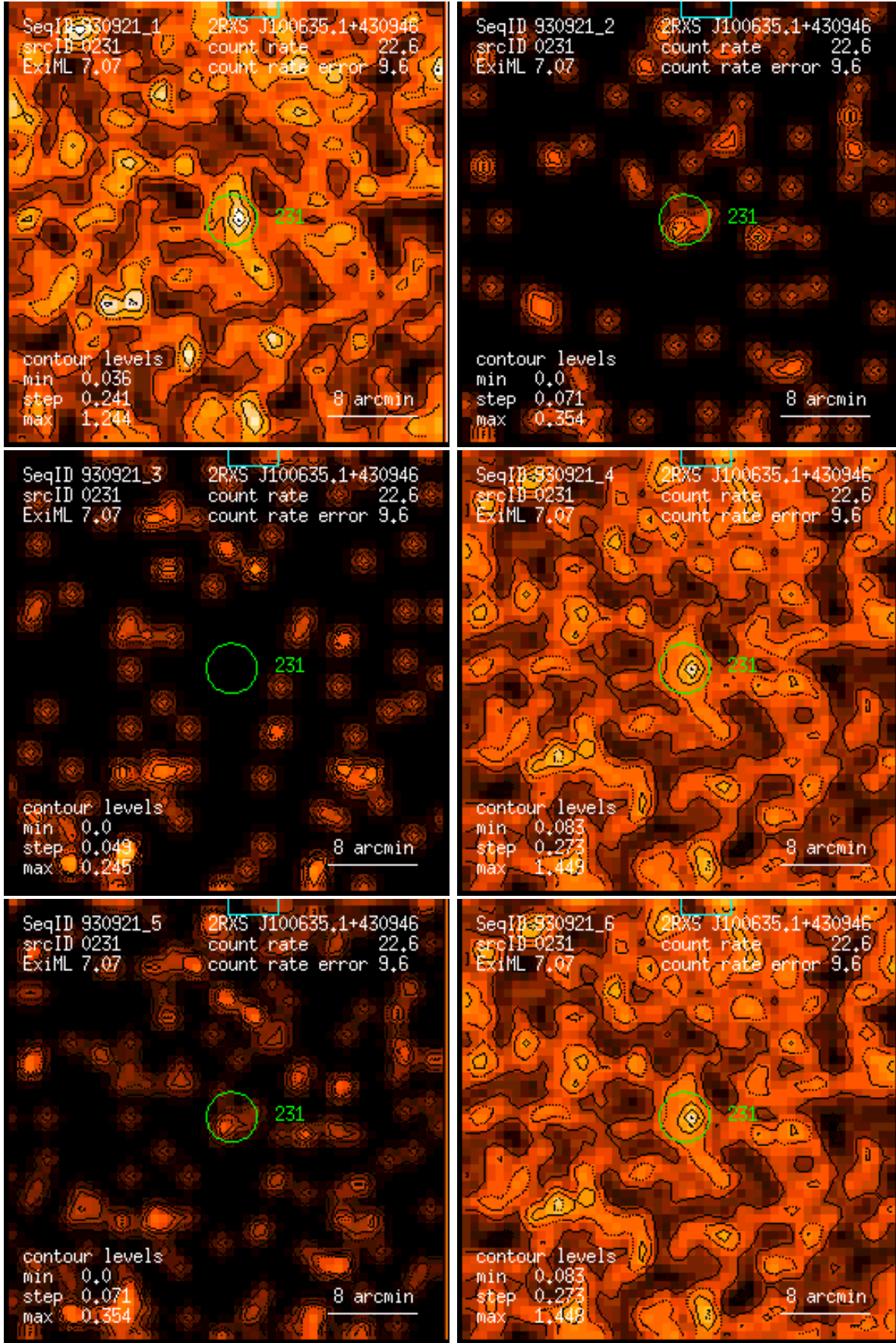
Figure 231: RASS 930921: detection 0231: band rate images, Gaussian filter: (1) PSPC channels 11 – 41, (2) 52 – 90, (3) 91 – 201, (4) 11 – 235, (5) 52 – 201, (6) 11 – 201. Broad band rates in counts/ks. Band rate contour levels in counts/ks/arcmin 2 .
