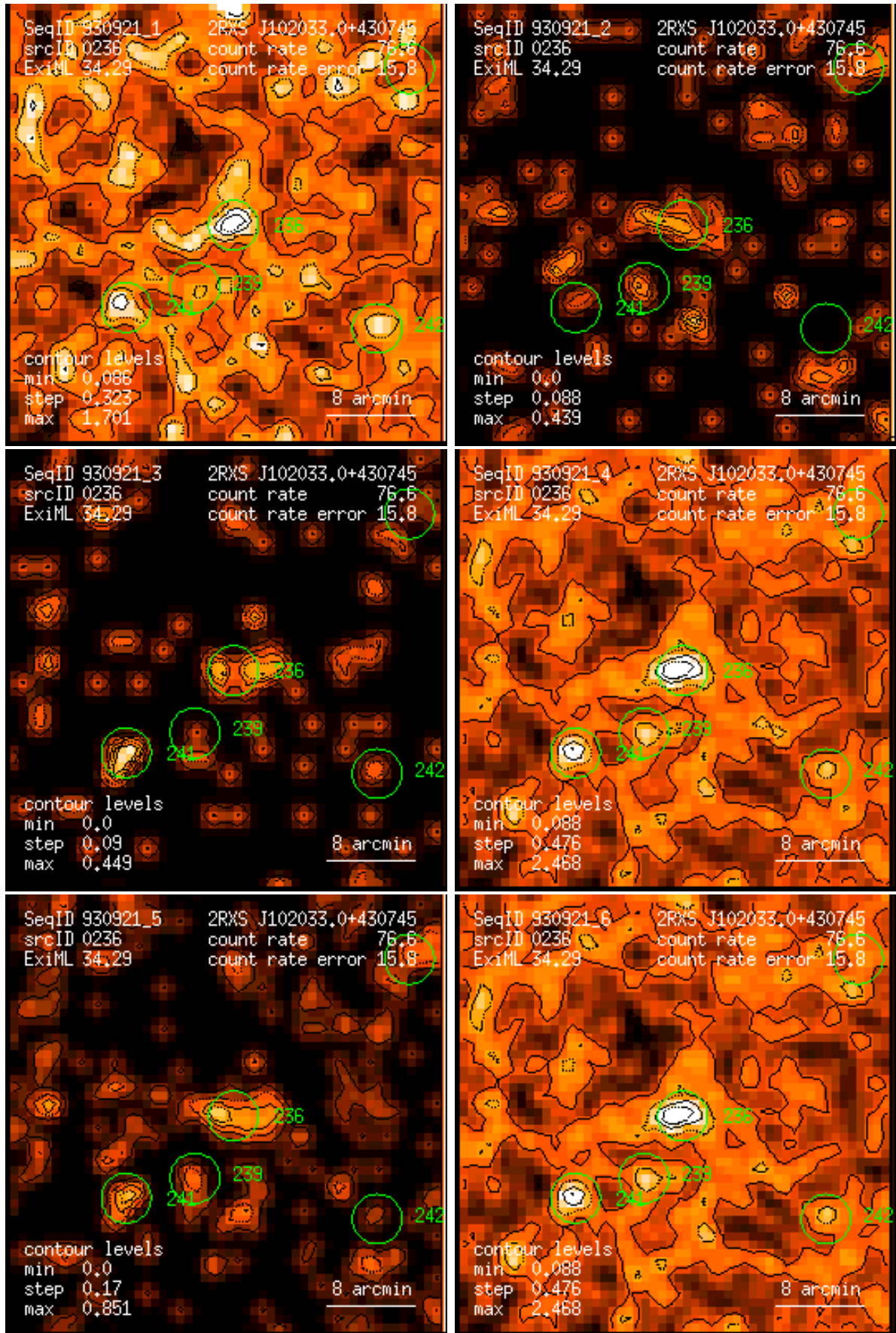
Figure 236: RASS 930921: detection 0236: band rate images, Gaussian filter: (1) PSPC channels 11 – 41, (2) 52 – 90, (3) 91 – 201, (4) 11 – 235, (5) 52 – 201, (6) 11 – 201. Broad band rates in counts/ks. Band rate contour levels in counts/ks/arcmin 2 .
