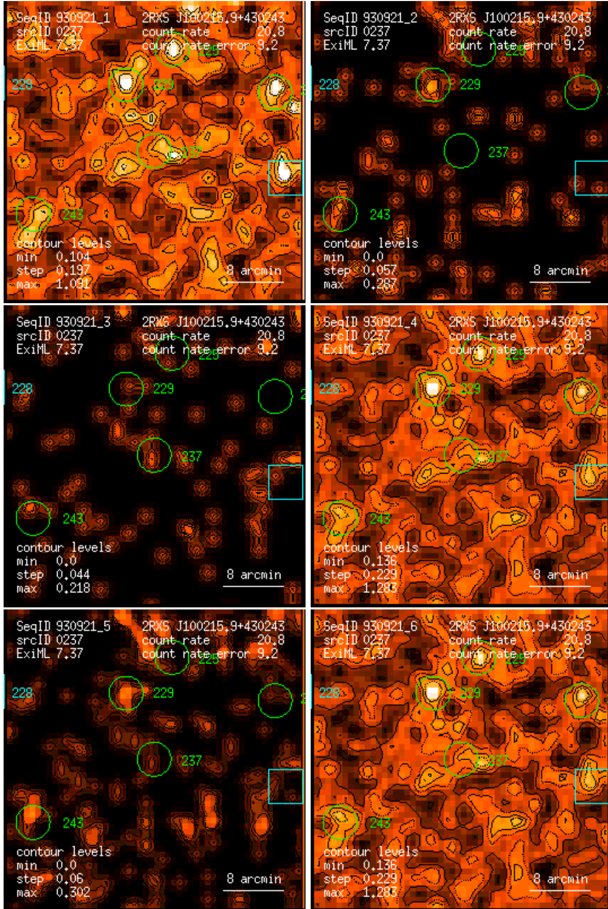
Figure 237: RASS 930921: detection 0237: band rate images, Gaussian filter: (1) PSPC channels 11 – 41, (2) 52 – 90, (3) 91 – 201, (4) 11 – 235, (5) 52 – 201, (6) 11 – 201. Broad band rates in counts/ks. Band rate contour levels in counts/ks/arcmin 2 .
