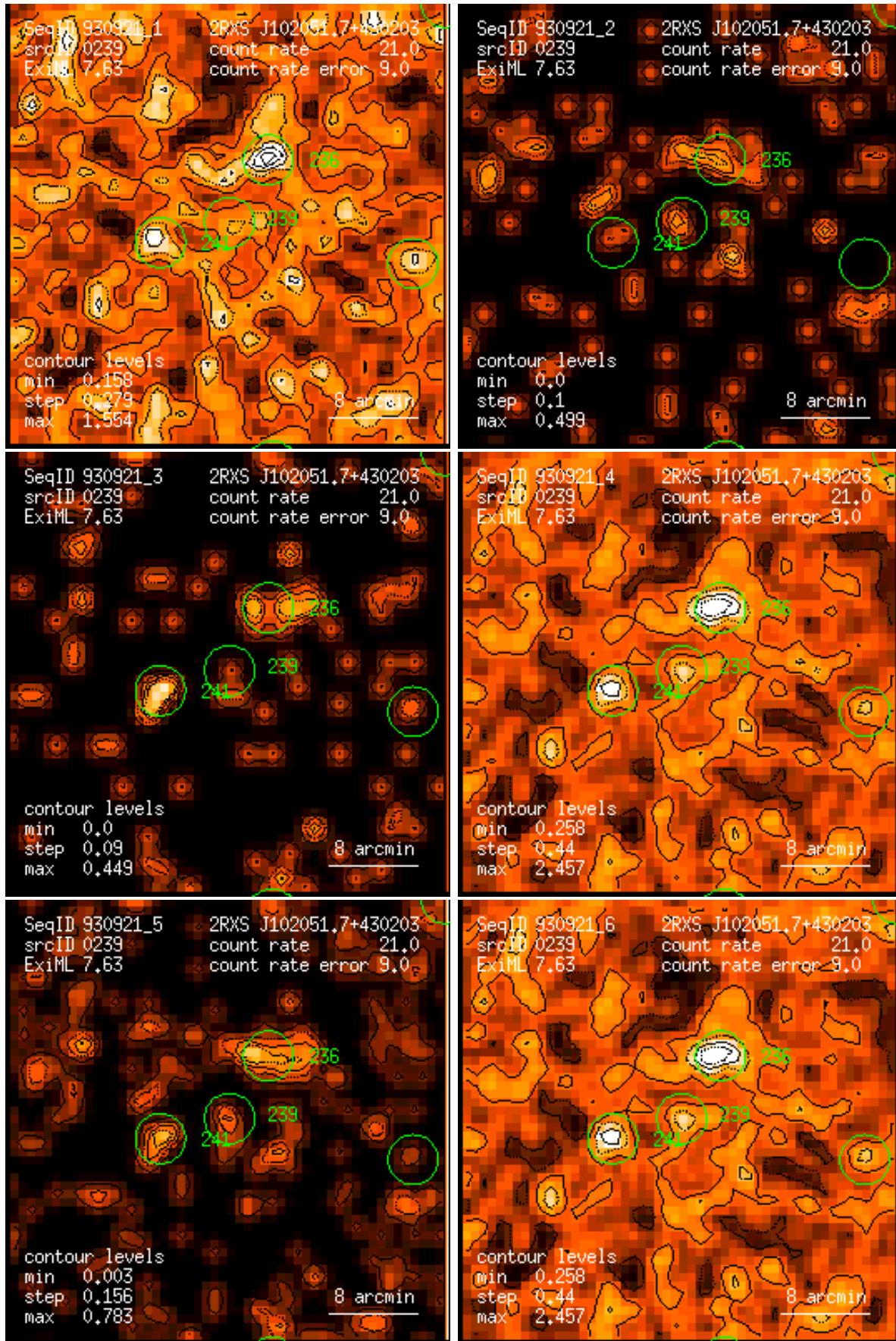
Figure 239: RASS 930921: detection 0239: band rate images, Gaussian filter: (1) PSPC channels 11 – 41, (2) 52 – 90, (3) 91 – 201, (4) 11 – 235, (5) 52 – 201, (6) 11 – 201. Broad band rates in counts/ks. Band rate contour levels in counts/ks/arcmin 2 .
