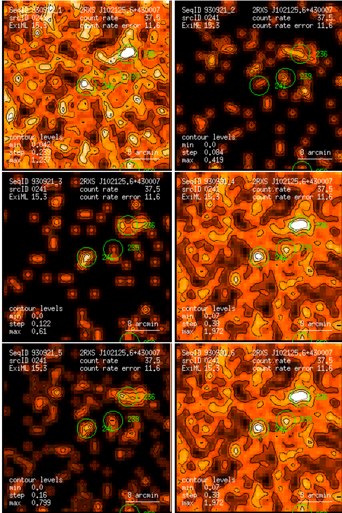
Figure 241: RASS 930921: detection 0241: band rate images, Gaussian filter: (1) PSPC channels 11 – 41, (2) 52 – 90, (3) 91 – 201, (4) 11 – 235, (5) 52 – 201, (6) 11 – 201. Broad band rates in counts/ks. Band rate contour levels in counts/ks/arcmin 2 .
