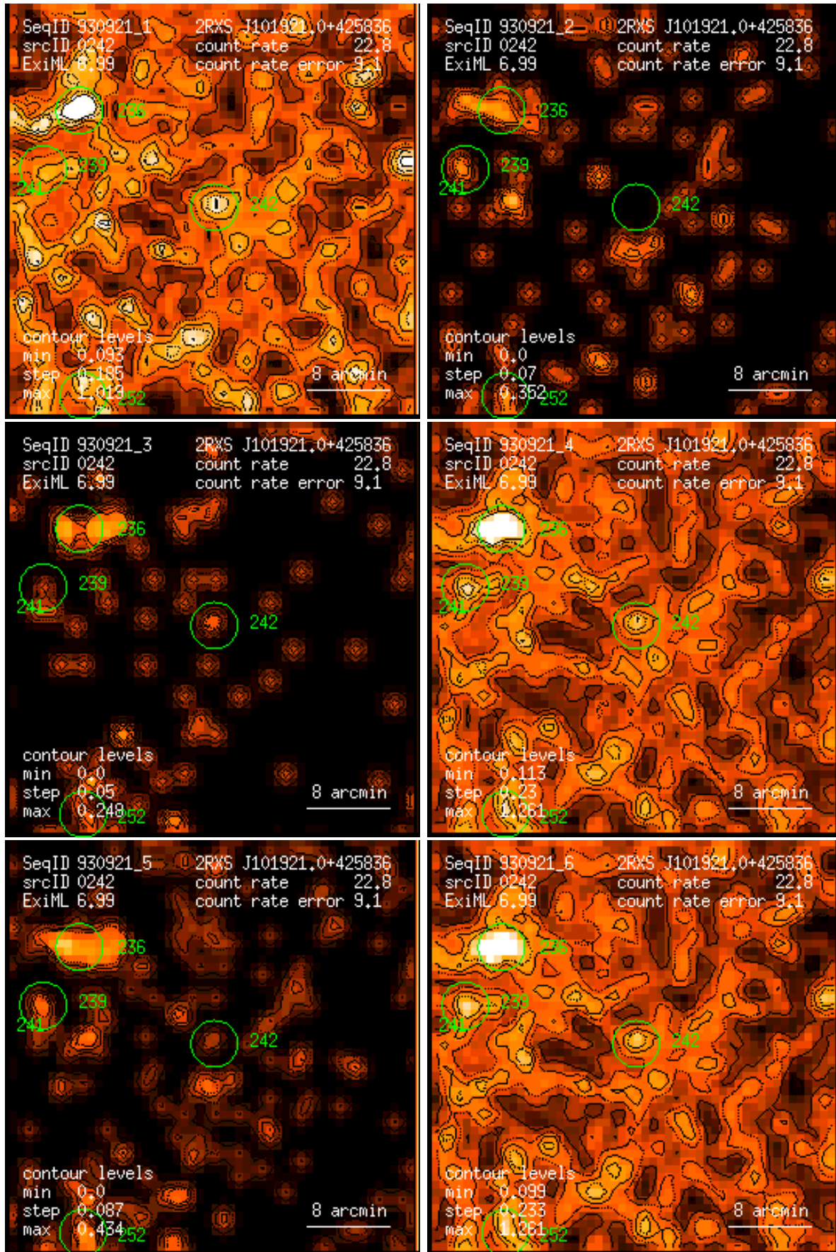
Figure 242: RASS 930921: detection 0242: band rate images, Gaussian filter: (1) PSPC channels 11 – 41, (2) 52 – 90, (3) 91 – 201, (4) 11 – 235, (5) 52 – 201, (6) 11 – 201. Broad band rates in counts/ks. Band rate contour levels in counts/ks/arcmin 2 .
