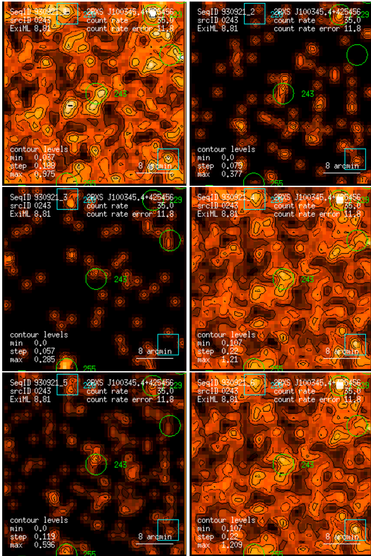
Figure 243: RASS 930921: detection 0243: band rate images, Gaussian filter: (1) PSPC channels 11 – 41, (2) 52 – 90, (3) 91 – 201, (4) 11 – 235, (5) 52 – 201, (6) 11 – 201. Broad band rates in counts/ks. Band rate contour levels in counts/ks/arcmin 2 .
