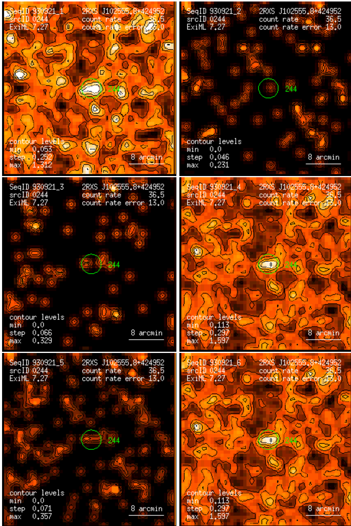
Figure 244: RASS 930921: detection 0244: band rate images, Gaussian filter: (1) PSPC channels 11 – 41, (2) 52 – 90, (3) 91 – 201, (4) 11 – 235, (5) 52 – 201, (6) 11 – 201. Broad band rates in counts/ks. Band rate contour levels in counts/ks/arcmin 2 .
