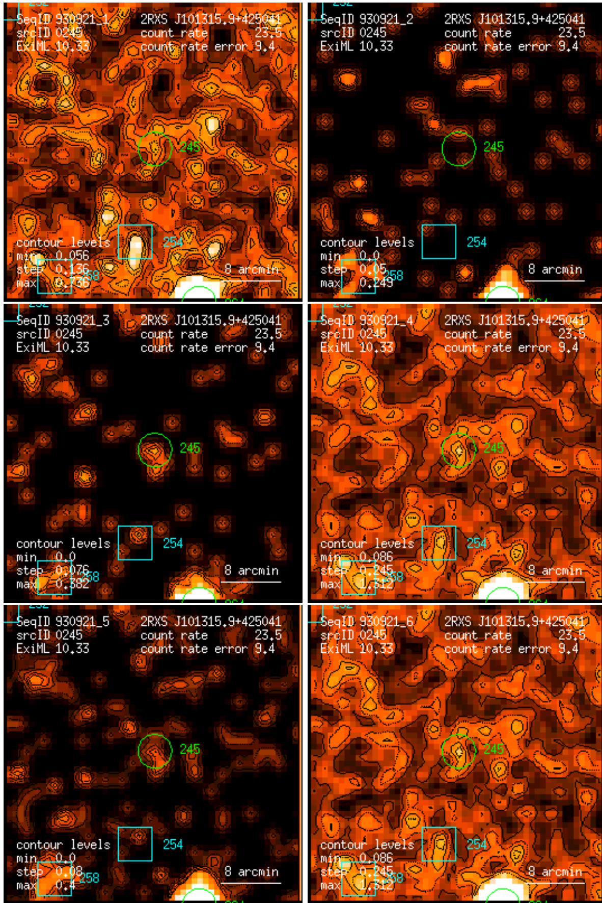
Figure 245: RASS 930921: detection 0245: band rate images, Gaussian filter: (1) PSPC channels 11 – 41, (2) 52 – 90, (3) 91 – 201, (4) 11 – 235, (5) 52 – 201, (6) 11 – 201. Broad band rates in counts/ks. Band rate contour levels in counts/ks/arcmin 2 .
