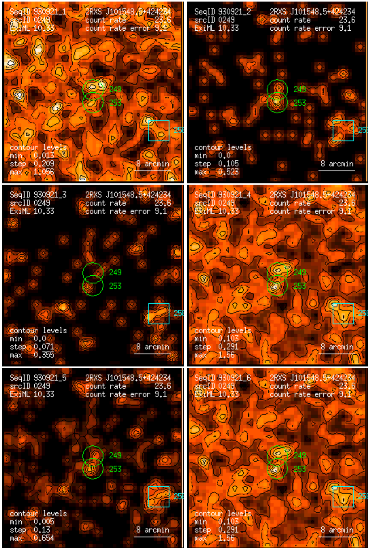
Figure 249: RASS 930921: detection 0249: band rate images, Gaussian filter: (1) PSPC channels 11 – 41, (2) 52 – 90, (3) 91 – 201, (4) 11 – 235, (5) 52 – 201, (6) 11 – 201. Broad band rates in counts/ks. Band rate contour levels in counts/ks/arcmin 2 .
