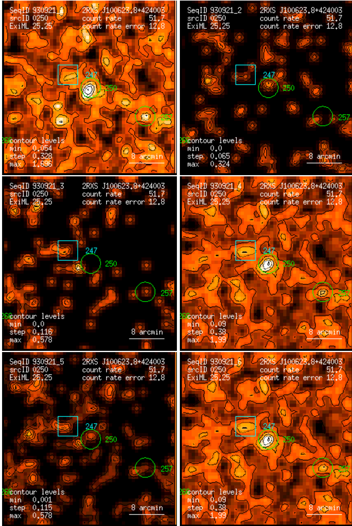
Figure 250: RASS 930921: detection 0250: band rate images, Gaussian filter: (1) PSPC channels 11 – 41, (2) 52 – 90, (3) 91 – 201, (4) 11 – 235, (5) 52 – 201, (6) 11 – 201. Broad band rates in counts/ks. Band rate contour levels in counts/ks/arcmin 2 .
