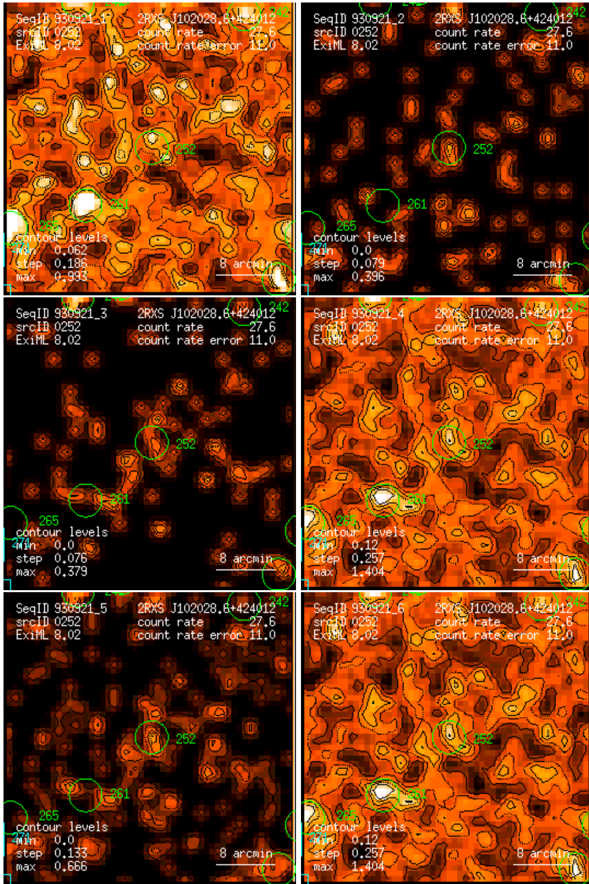
Figure 252: RASS 930921: detection 0252: band rate images, Gaussian filter: (1) PSPC channels 11 – 41, (2) 52 – 90, (3) 91 – 201, (4) 11 – 235, (5) 52 – 201, (6) 11 – 201. Broad band rates in counts/ks. Band rate contour levels in counts/ks/arcmin 2 .
