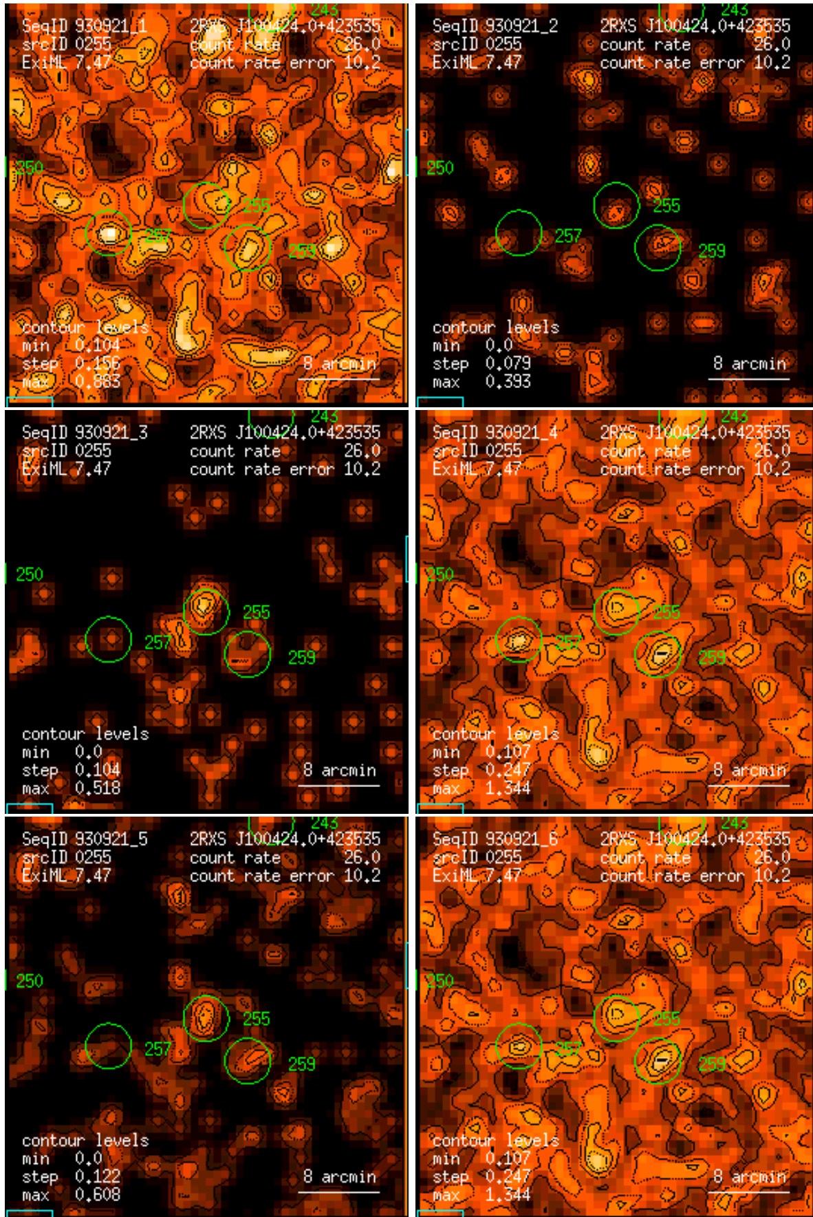
Figure 255: RASS 930921: detection 0255: band rate images, Gaussian filter: (1) PSPC channels 11 – 41, (2) 52 – 90, (3) 91 – 201, (4) 11 – 235, (5) 52 – 201, (6) 11 – 201. Broad band rates in counts/ks. Band rate contour levels in counts/ks/arcmin 2 .
