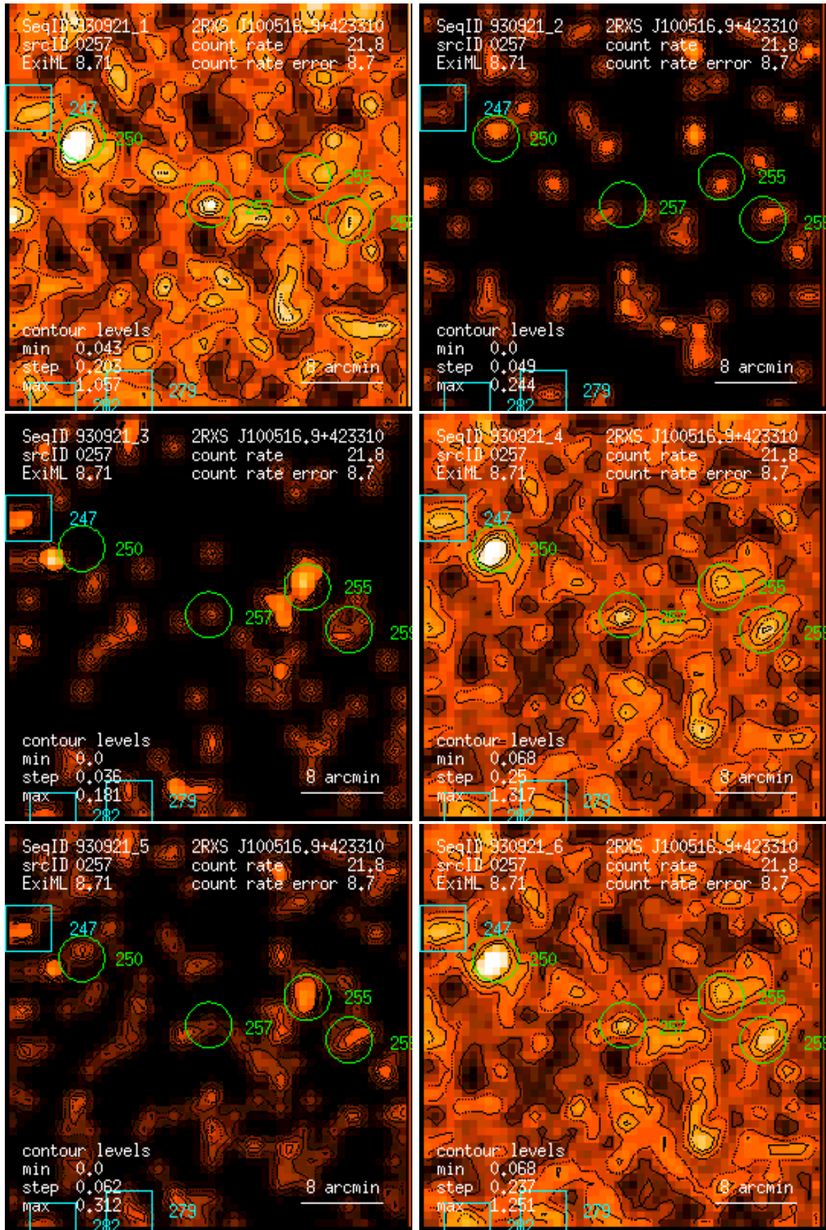
Figure 257: RASS 930921: detection 0257: band rate images, Gaussian filter: (1) PSPC channels 11 – 41, (2) 52 – 90, (3) 91 – 201, (4) 11 – 235, (5) 52 – 201, (6) 11 – 201. Broad band rates in counts/ks. Band rate contour levels in counts/ks/arcmin 2 .
