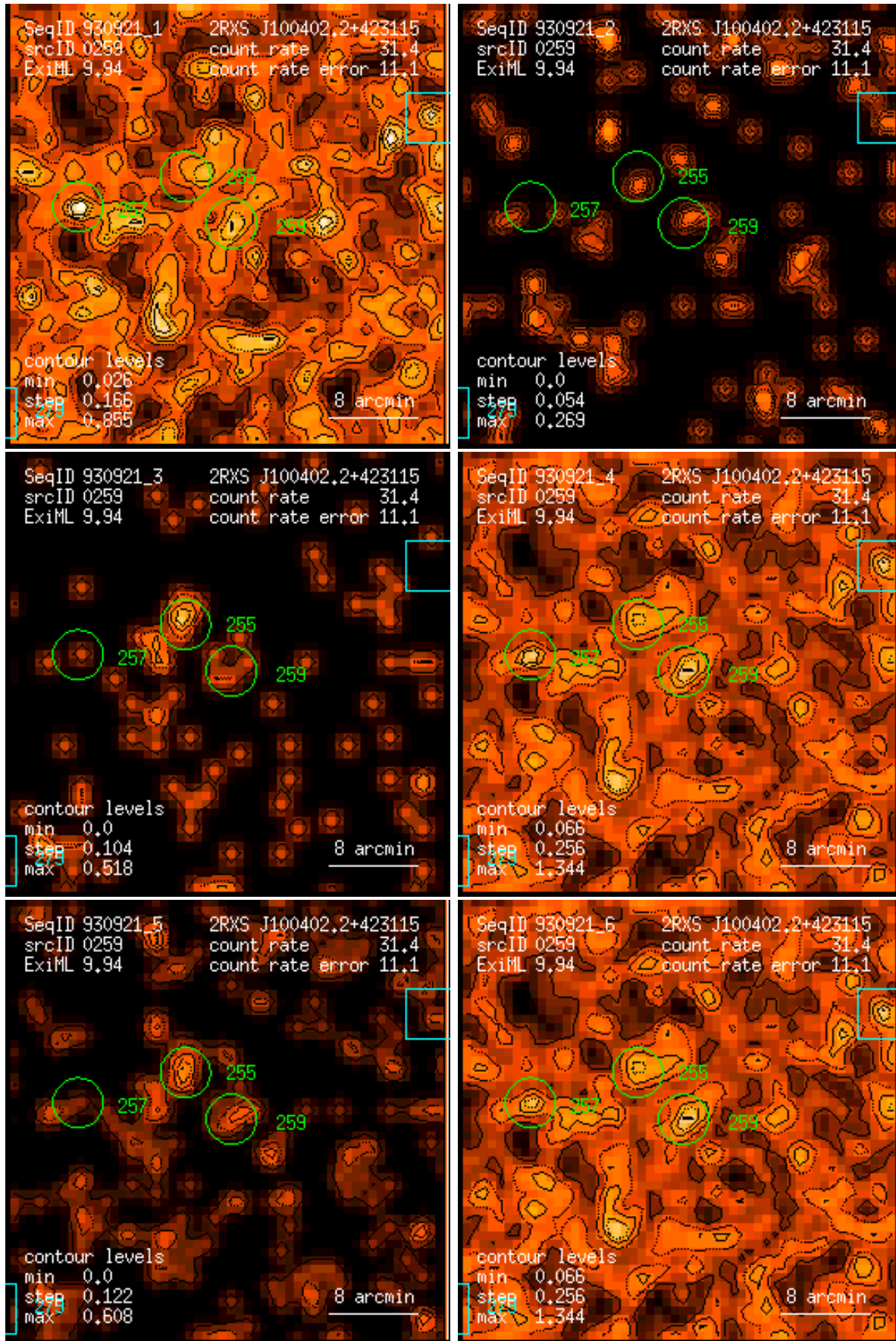
Figure 259: RASS 930921: detection 0259: band rate images, Gaussian filter: (1) PSPC channels 11 – 41, (2) 52 – 90, (3) 91 – 201, (4) 11 – 235, (5) 52 – 201, (6) 11 – 201. Broad band rates in counts/ks. Band rate contour levels in counts/ks/arcmin 2 .
