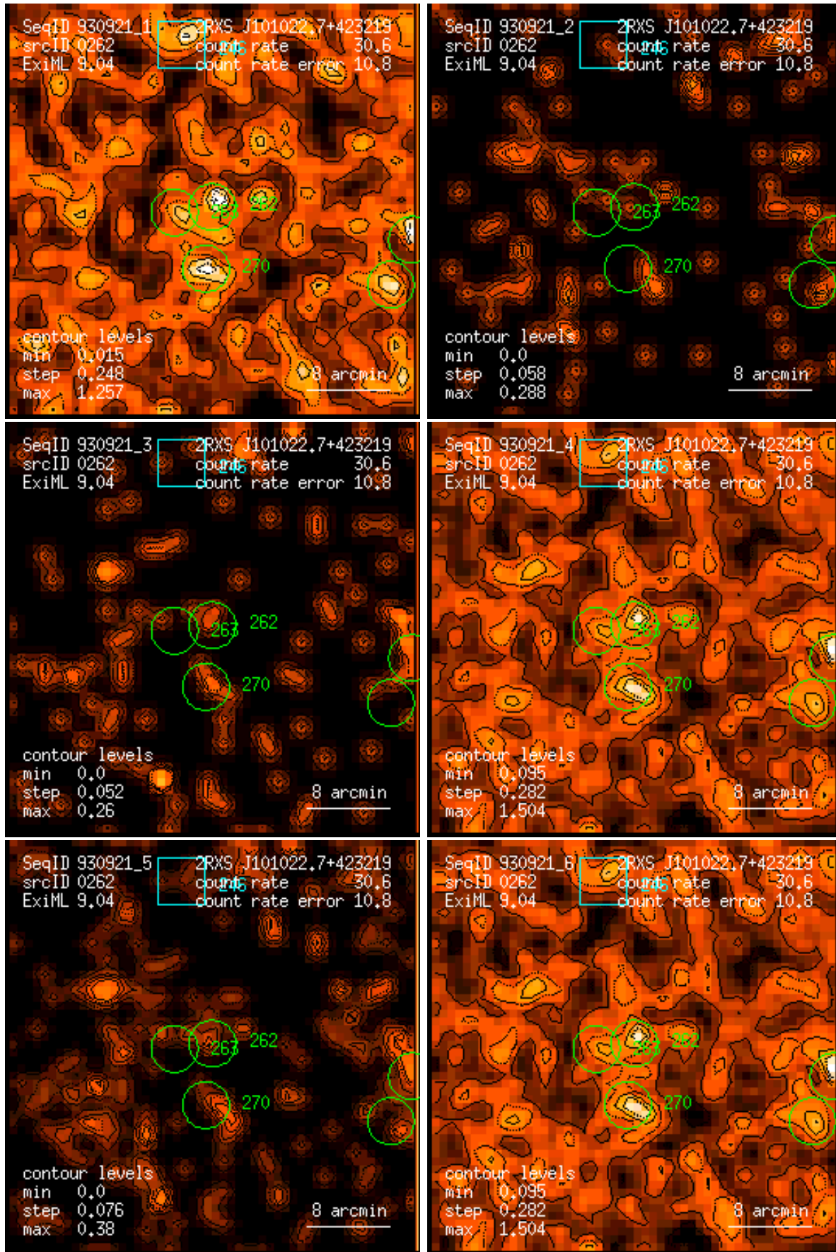
Figure 262: RASS 930921: detection 0262: band rate images, Gaussian filter: (1) PSPC channels 11 – 41, (2) 52 – 90, (3) 91 – 201, (4) 11 – 235, (5) 52 – 201, (6) 11 – 201. Broad band rates in counts/ks. Band rate contour levels in counts/ks/arcmin 2 .
