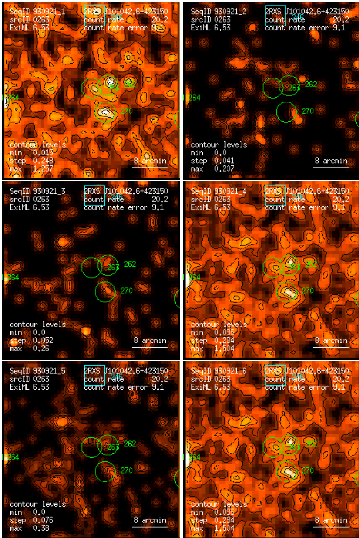
Figure 263: RASS 930921: detection 0263: band rate images, Gaussian filter: (1) PSPC channels 11 – 41, (2) 52 – 90, (3) 91 – 201, (4) 11 – 235, (5) 52 – 201, (6) 11 – 201. Broad band rates in counts/ks. Band rate contour levels in counts/ks/arcmin 2 .
